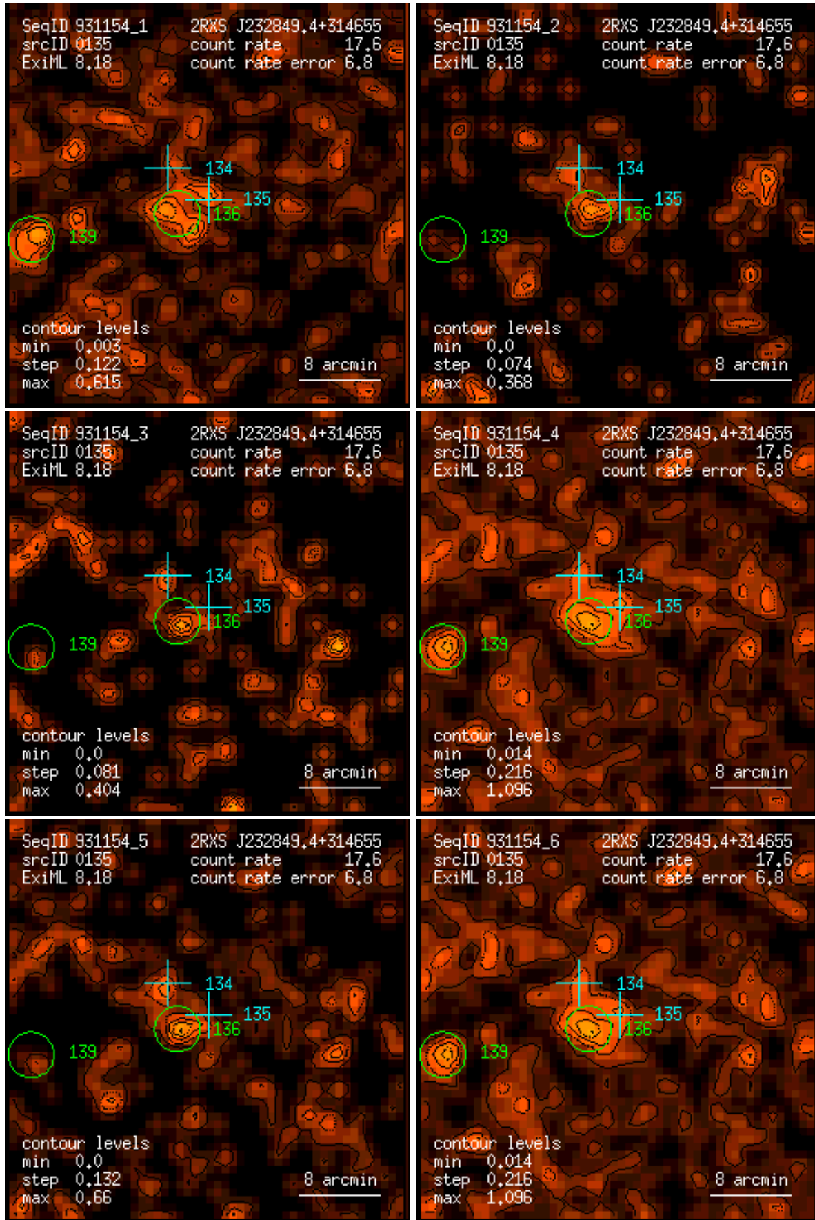
Figure 135: RASS 931154: detection 0135: band rate images, Gaussian filter: (1) PSPC channels 11 – 41, (2) 52 – 90, (3) 91 – 201, (4) 11 – 235, (5) 52 – 201, (6) 11 – 201. Broad band rates in counts/ks. Band rate contour levels in counts/ks/arcmin 2 .
