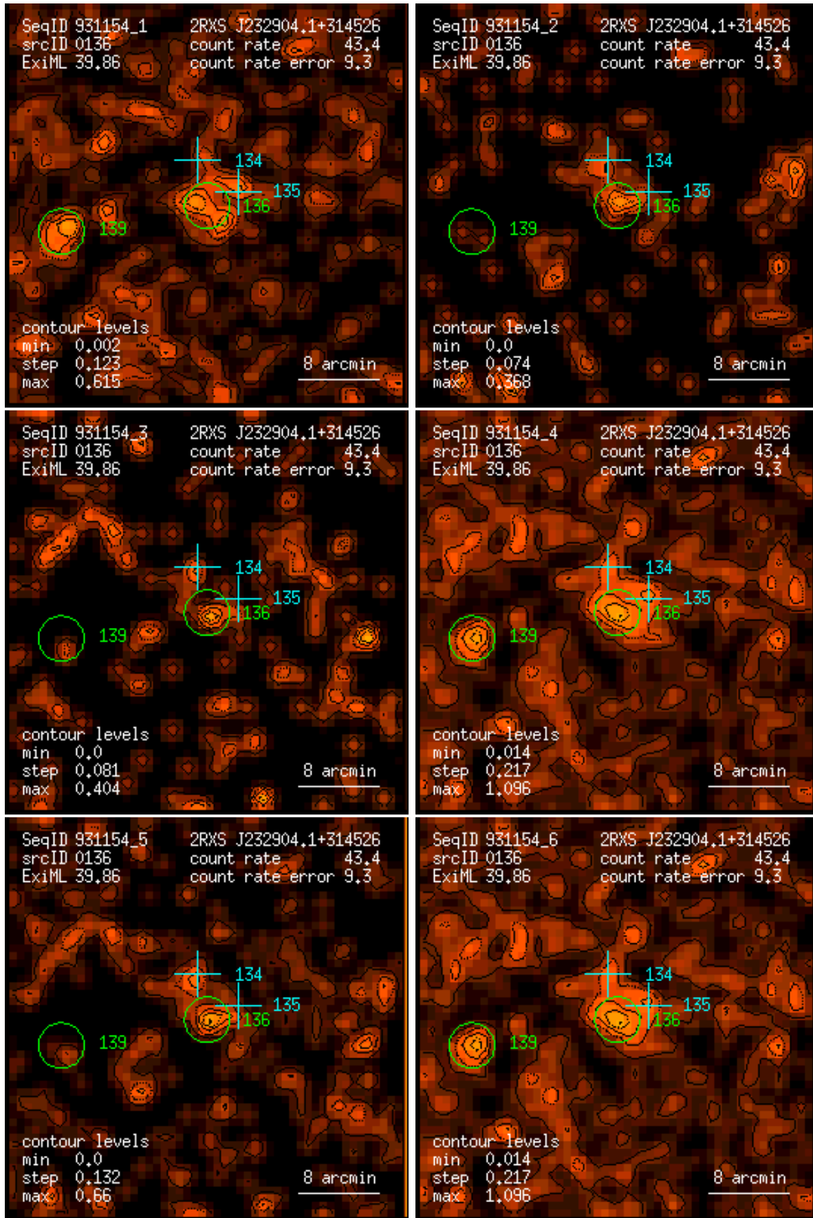
Figure 136: RASS 931154: detection 0136: band rate images, Gaussian filter: (1) PSPC channels 11 – 41, (2) 52 – 90, (3) 91 – 201, (4) 11 – 235, (5) 52 – 201, (6) 11 – 201. Broad band rates in counts/ks. Band rate contour levels in counts/ks/arcmin 2 .
