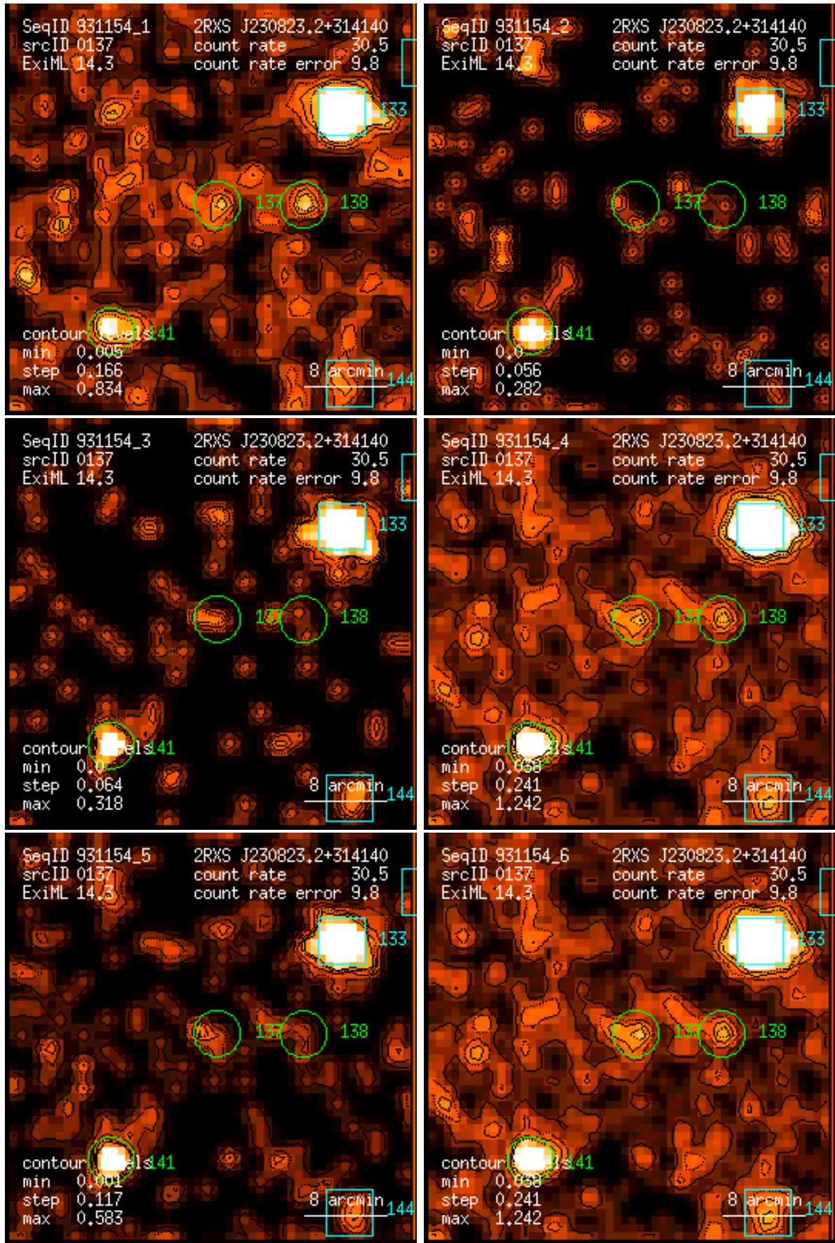
Figure 137: RASS 931154: detection 0137: band rate images, Gaussian filter: (1) PSPC channels 11 – 41, (2) 52 – 90, (3) 91 – 201, (4) 11 – 235, (5) 52 – 201, (6) 11 – 201. Broad band rates in counts/ks. Band rate contour levels in counts/ks/arcmin 2 .
