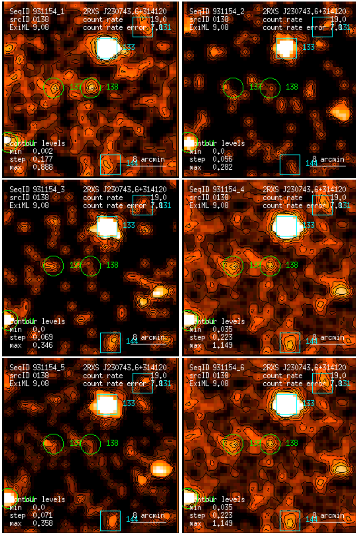
Figure 138: RASS 931154: detection 0138: band rate images, Gaussian filter: (1) PSPC channels 11 – 41, (2) 52 – 90, (3) 91 – 201, (4) 11 – 235, (5) 52 – 201, (6) 11 – 201. Broad band rates in counts/ks. Band rate contour levels in counts/ks/arcmin 2 .
