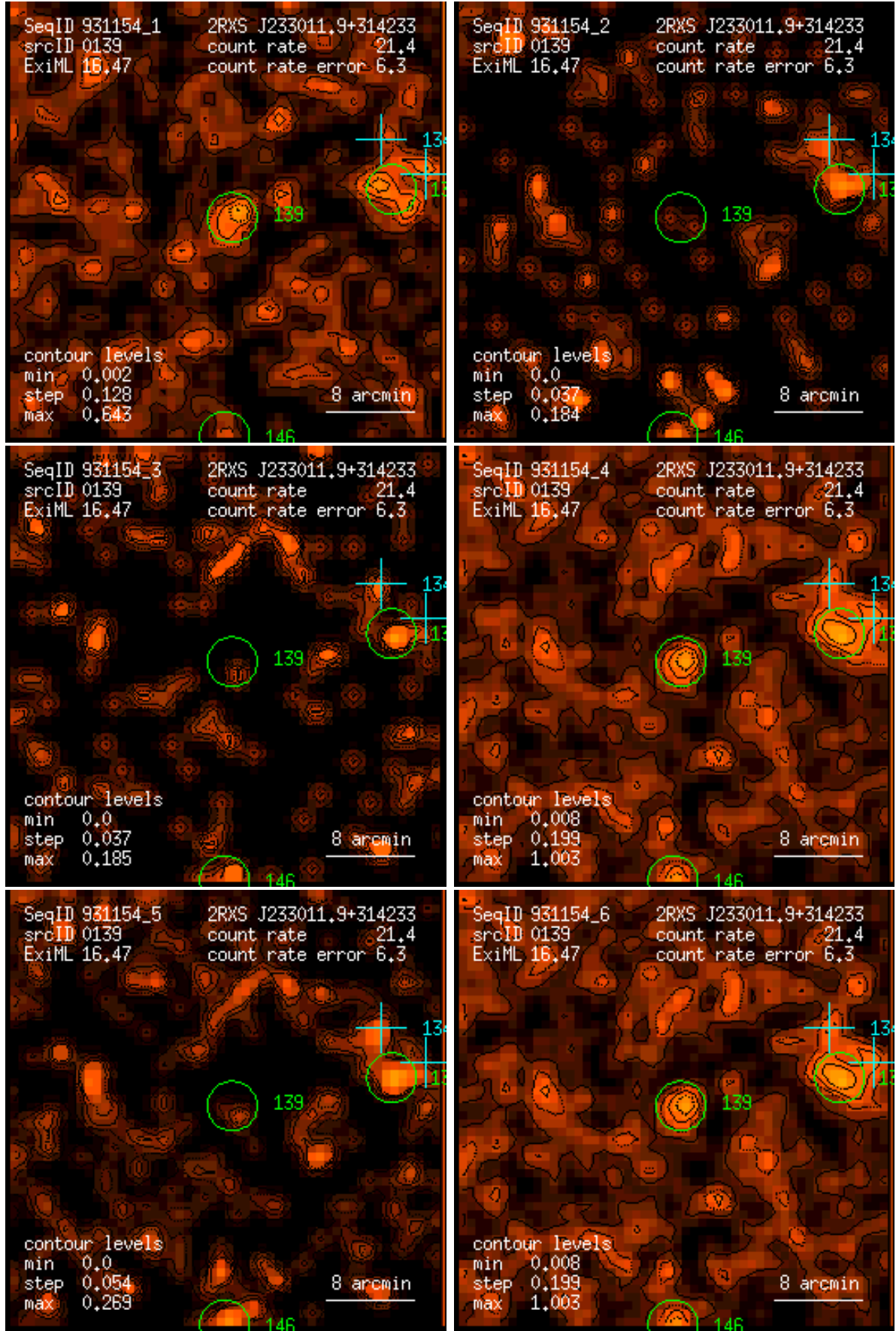
Figure 139: RASS 931154: detection 0139: band rate images, Gaussian filter: (1) PSPC channels 11 – 41, (2) 52 – 90, (3) 91 – 201, (4) 11 – 235, (5) 52 – 201, (6) 11 – 201. Broad band rates in counts/ks. Band rate contour levels in counts/ks/arcmin 2 .
