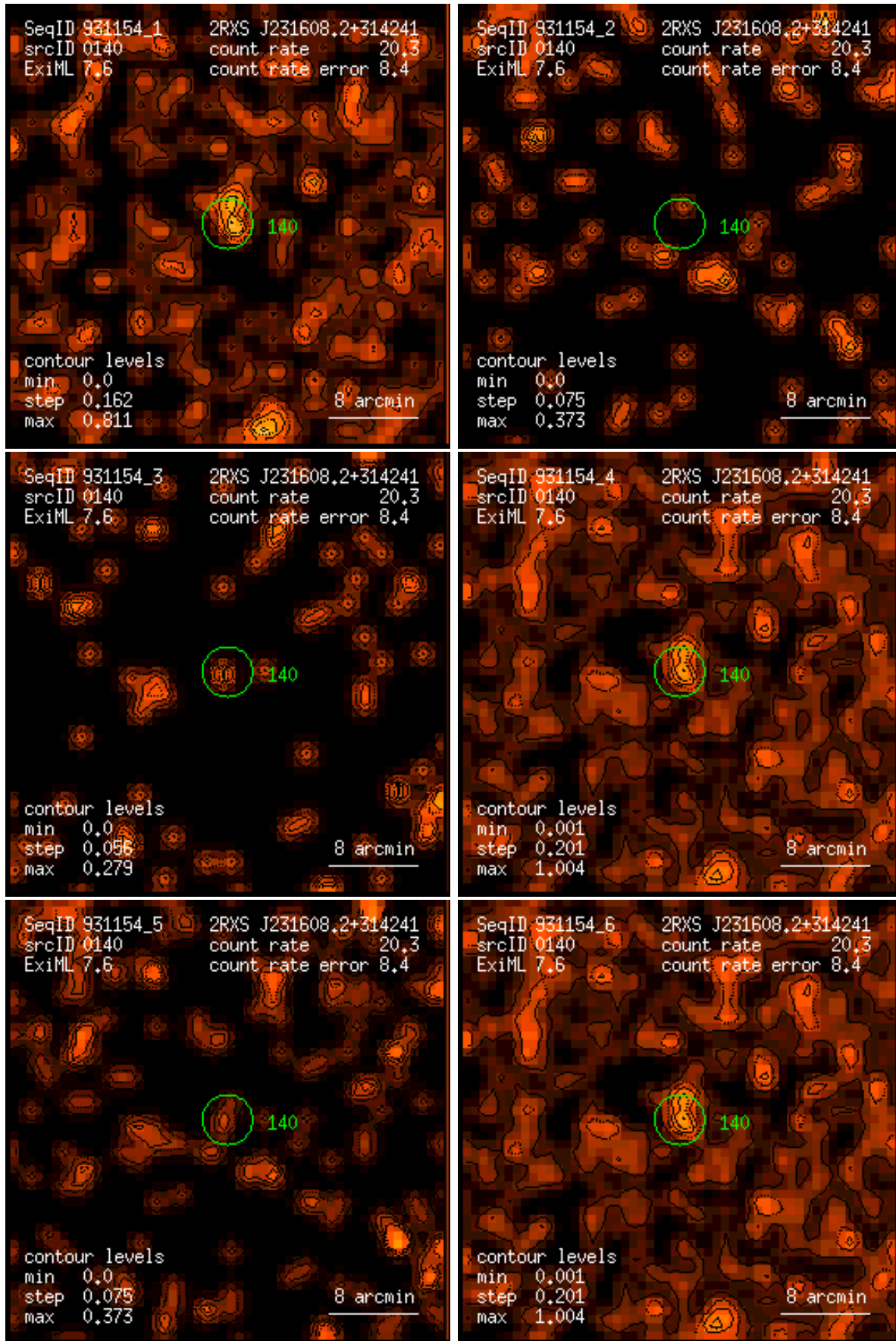
Figure 140: RASS 931154: detection 0140: band rate images, Gaussian filter: (1) PSPC channels 11 – 41, (2) 52 – 90, (3) 91 – 201, (4) 11 – 235, (5) 52 – 201, (6) 11 – 201. Broad band rates in counts/ks. Band rate contour levels in counts/ks/arcmin 2 .
