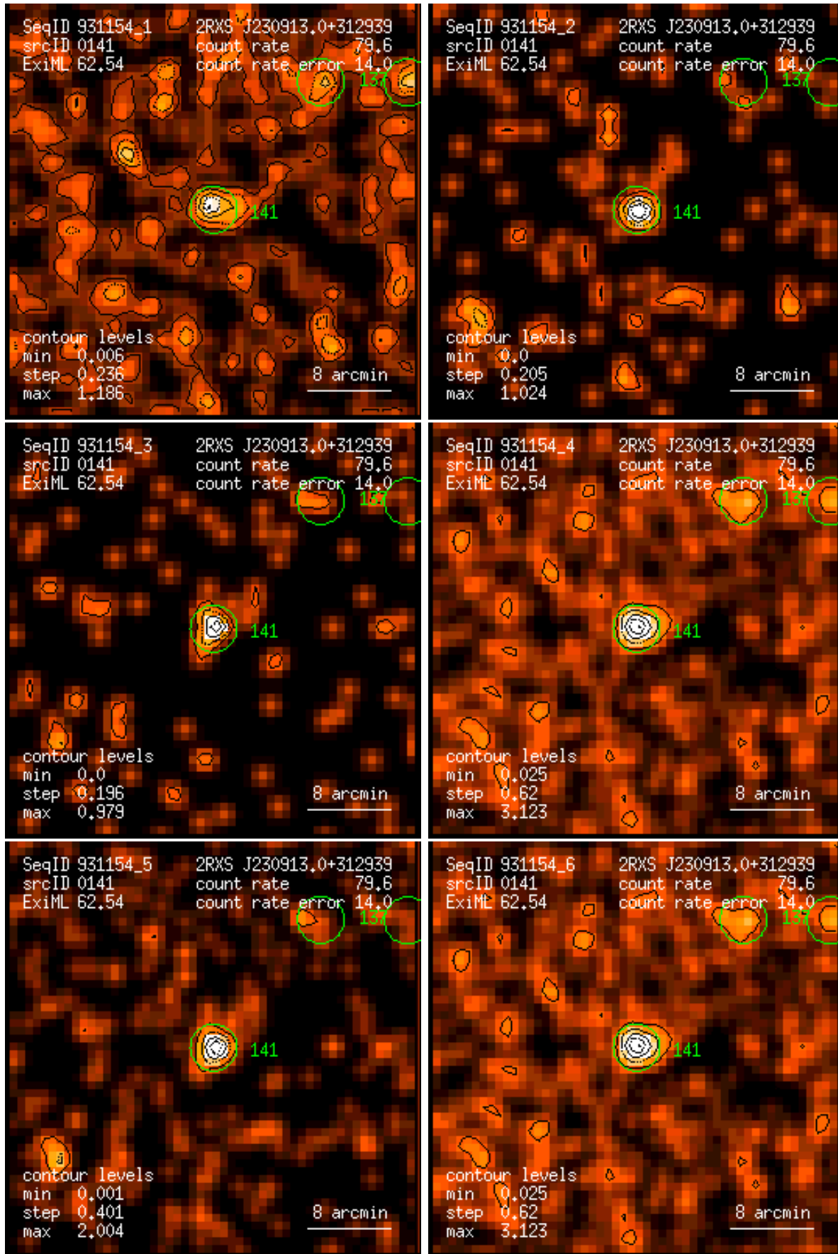
Figure 141: RASS 931154: detection 0141: band rate images, Gaussian filter: (1) PSPC channels 11 – 41, (2) 52 – 90, (3) 91 – 201, (4) 11 – 235, (5) 52 – 201, (6) 11 – 201. Broad band rates in counts/ks. Band rate contour levels in counts/ks/arcmin 2 .
