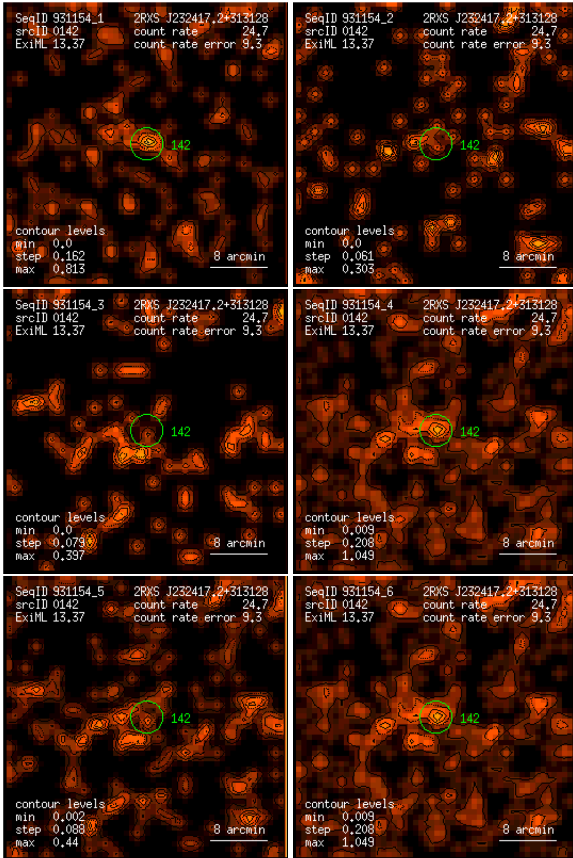
Figure 142: RASS 931154: detection 0142: band rate images, Gaussian filter: (1) PSPC channels 11 – 41, (2) 52 – 90, (3) 91 – 201, (4) 11 – 235, (5) 52 – 201, (6) 11 – 201. Broad band rates in counts/ks. Band rate contour levels in counts/ks/arcmin 2 .
