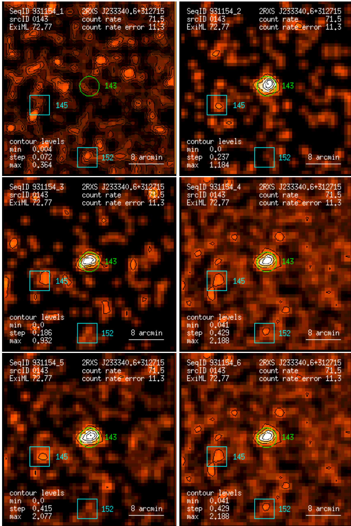
Figure 143: RASS 931154: detection 0143: band rate images, Gaussian filter: (1) PSPC channels 11 – 41, (2) 52 – 90, (3) 91 – 201, (4) 11 – 235, (5) 52 – 201, (6) 11 – 201. Broad band rates in counts/ks. Band rate contour levels in counts/ks/arcmin 2 .
