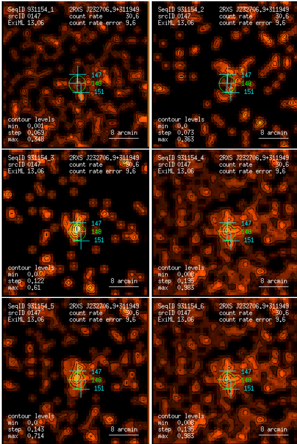
Figure 147: RASS 931154: detection 0147: band rate images, Gaussian filter: (1) PSPC channels 11 – 41, (2) 52 – 90, (3) 91 – 201, (4) 11 – 235, (5) 52 – 201, (6) 11 – 201. Broad band rates in counts/ks. Band rate contour levels in counts/ks/arcmin 2 .
