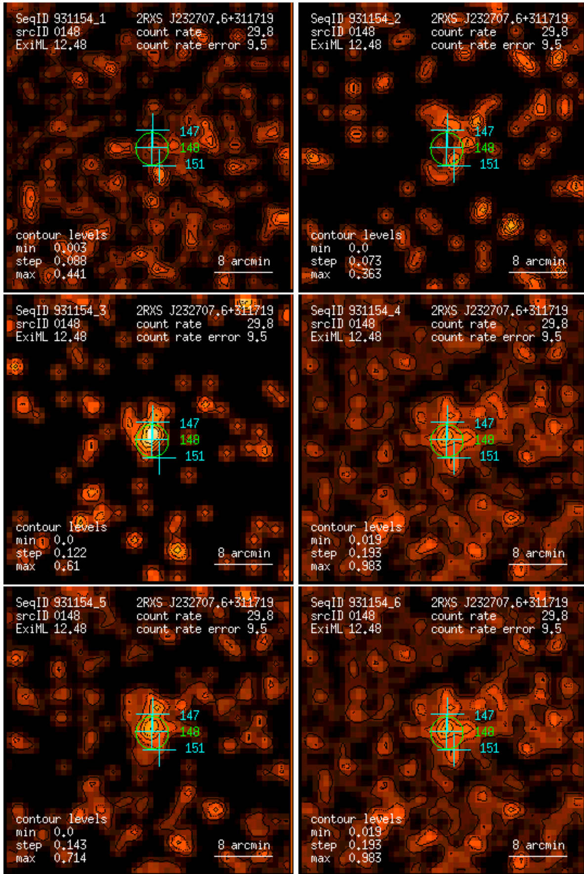
Figure 148: RASS 931154: detection 0148: band rate images, Gaussian filter: (1) PSPC channels 11 – 41, (2) 52 – 90, (3) 91 – 201, (4) 11 – 235, (5) 52 – 201, (6) 11 – 201. Broad band rates in counts/ks. Band rate contour levels in counts/ks/arcmin 2 .
