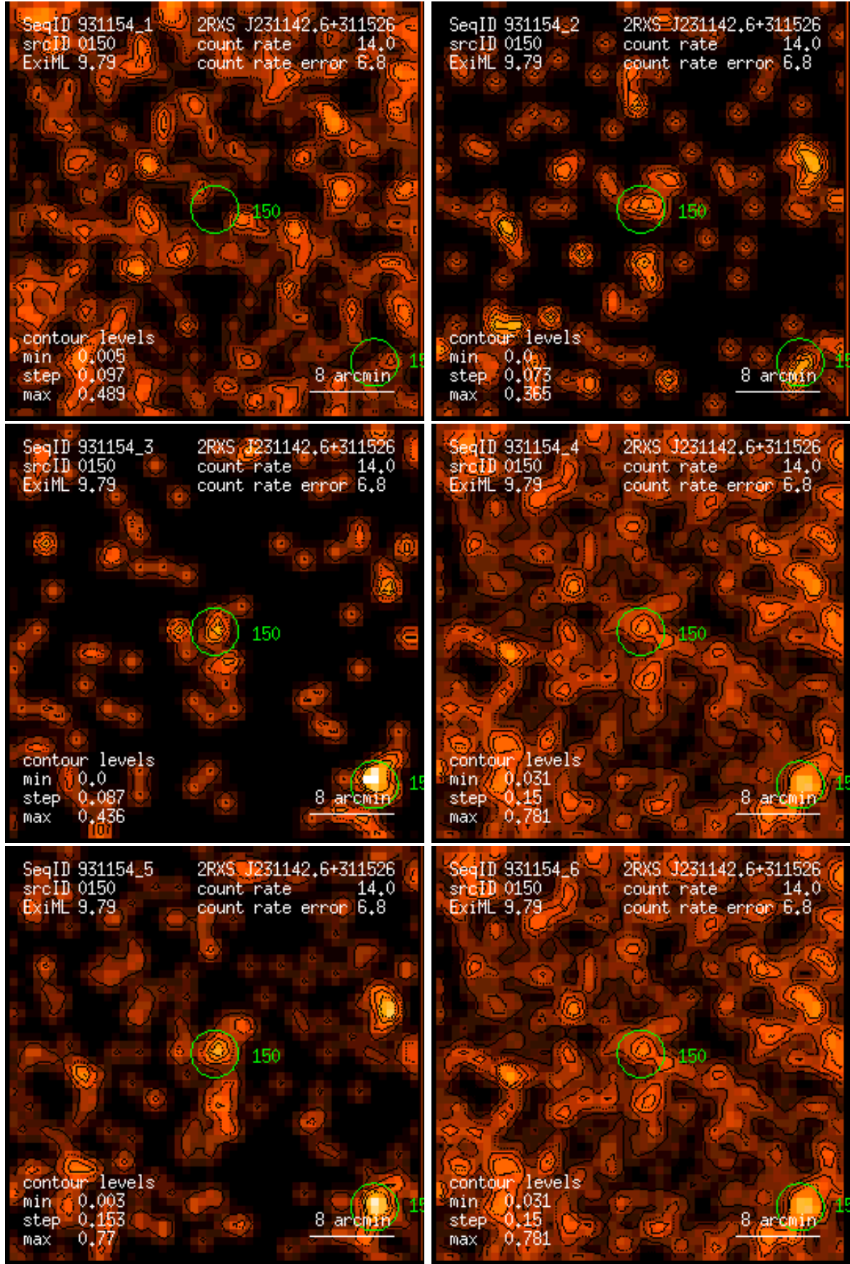
Figure 150: RASS 931154: detection 0150: band rate images, Gaussian filter: (1) PSPC channels 11 – 41, (2) 52 – 90, (3) 91 – 201, (4) 11 – 235, (5) 52 – 201, (6) 11 – 201. Broad band rates in counts/ks. Band rate contour levels in counts/ks/arcmin 2 .
