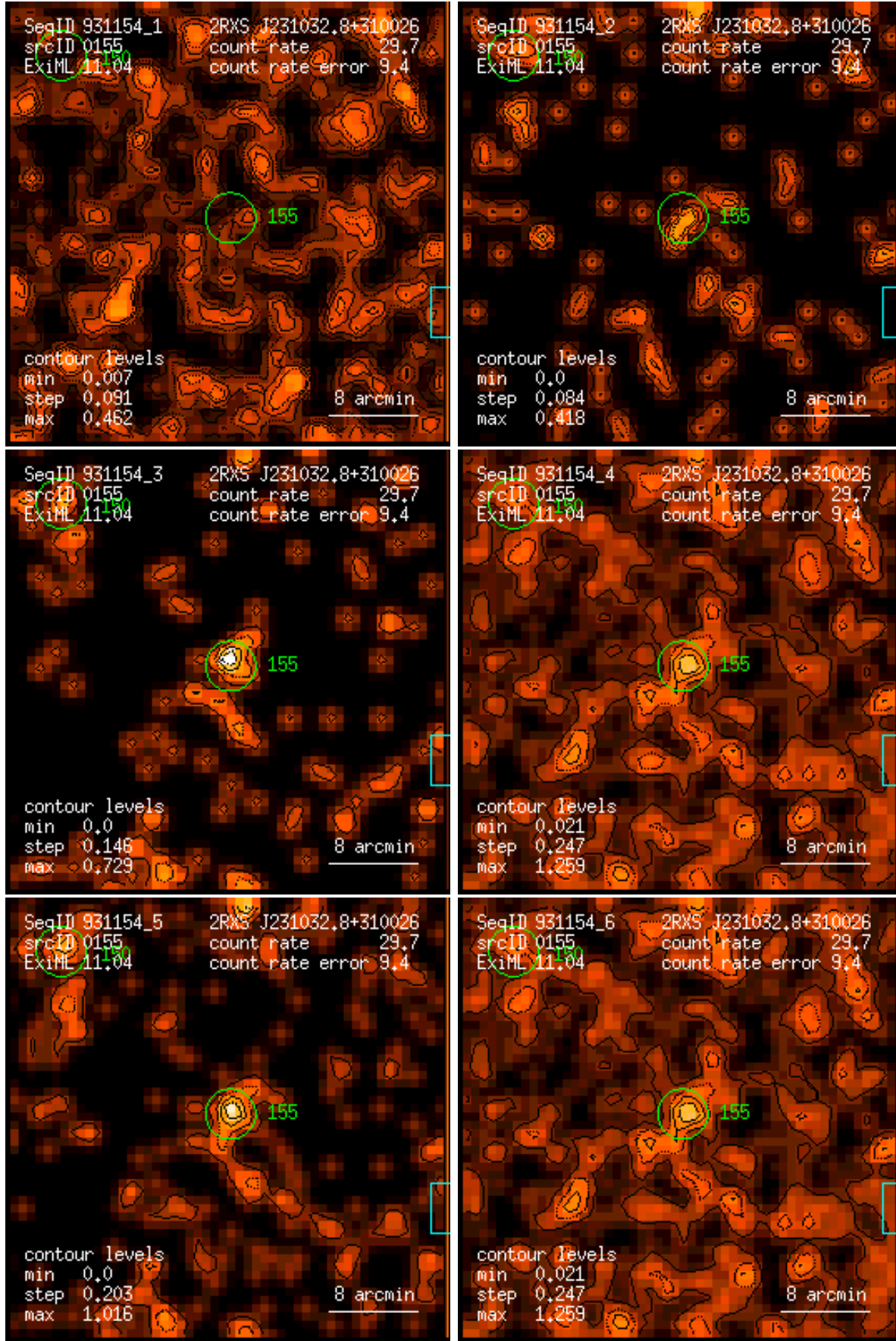
Figure 155: RASS 931154: detection 0155: band rate images, Gaussian filter: (1) PSPC channels 11 – 41, (2) 52 – 90, (3) 91 – 201, (4) 11 – 235, (5) 52 – 201, (6) 11 – 201. Broad band rates in counts/ks. Band rate contour levels in counts/ks/arcmin 2 .
