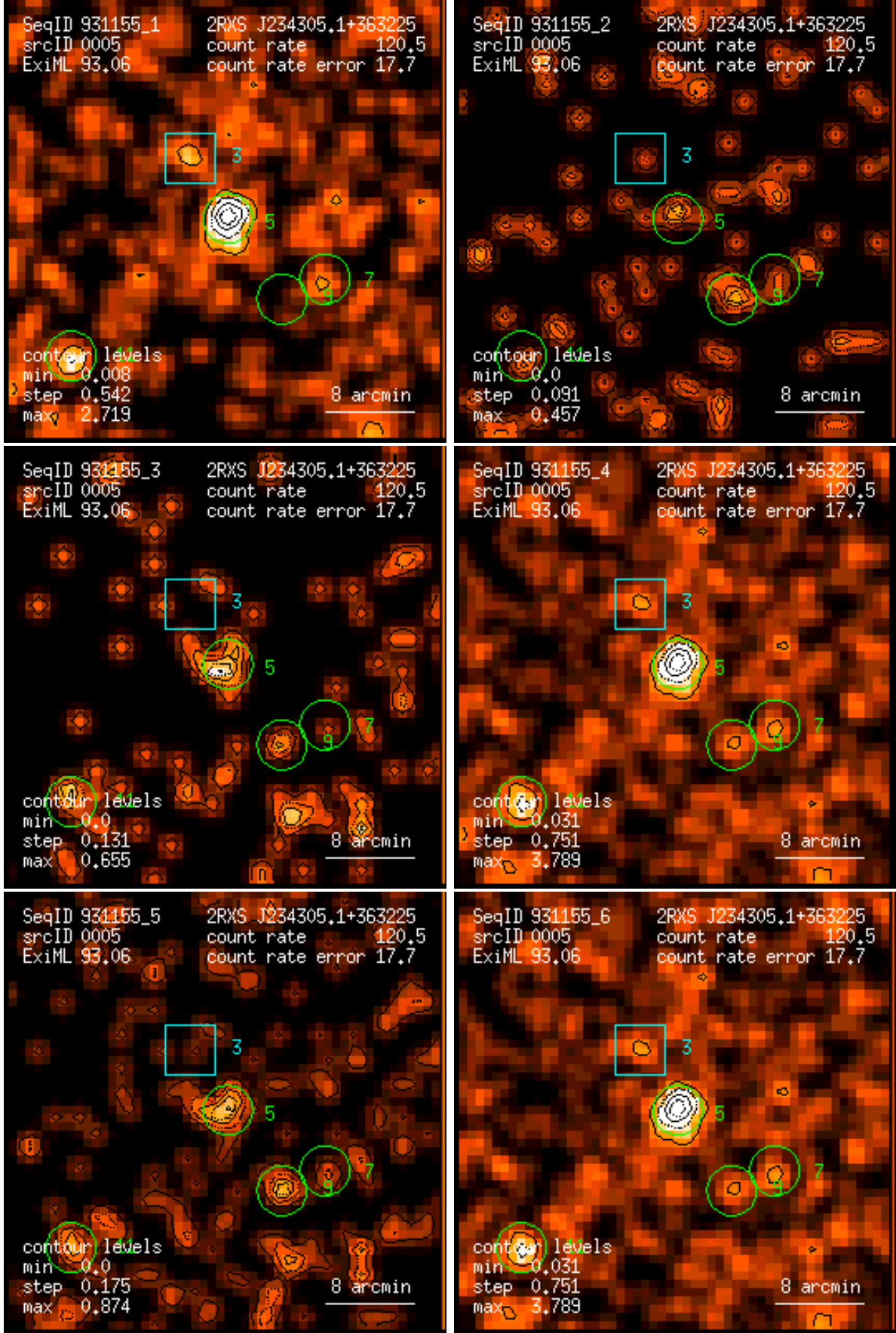
Figure 5: RASS 931155: detection 0005: band rate images, Gaussian filter: (1) PSPC channels 11 – 41, (2) 52 – 90, (3) 91 – 201, (4) 11 – 235, (5) 52 – 201, (6) 11 – 201. Broad band rates in counts/ks. Band rate contour levels in counts/ks/arcmin 2 .
