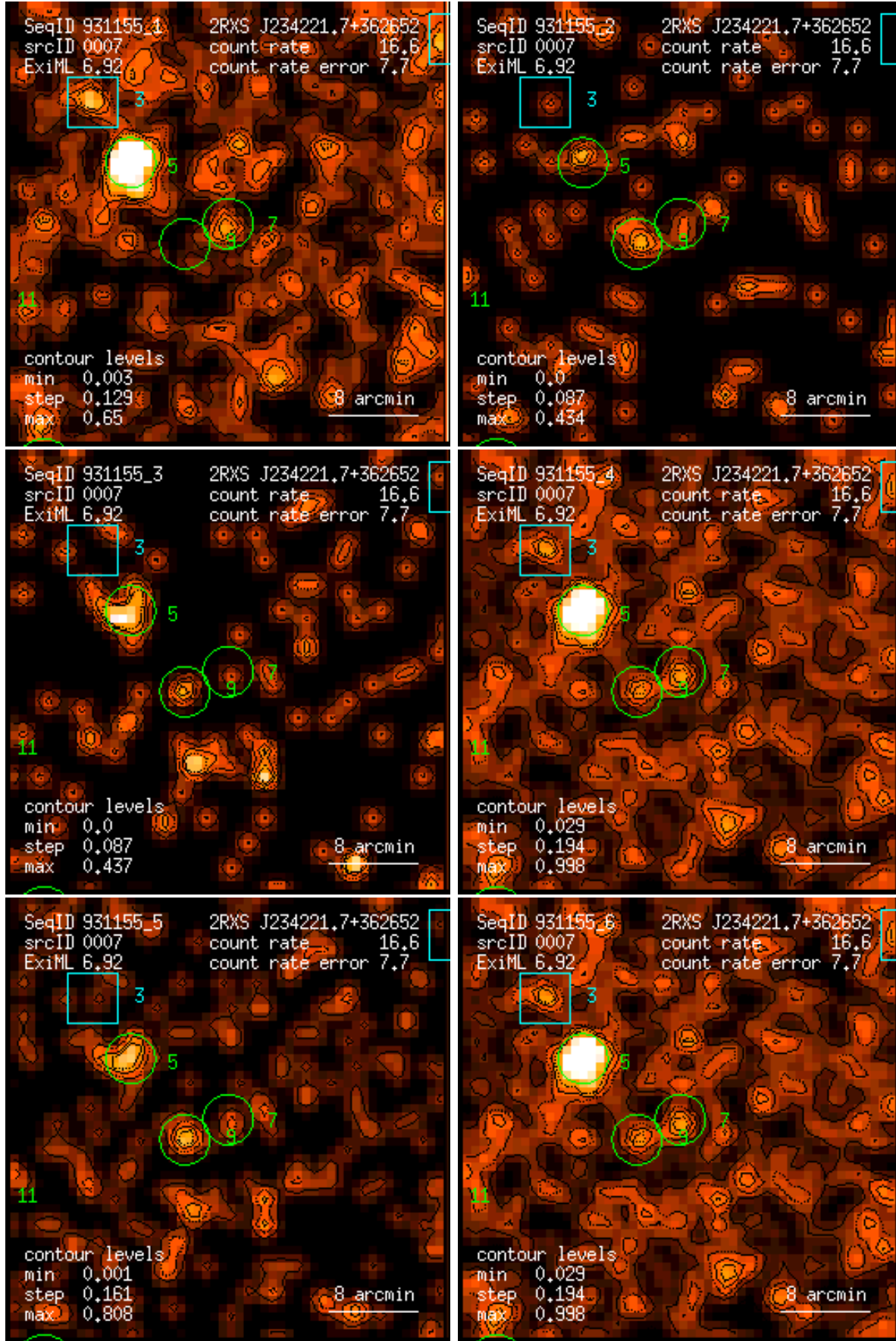
Figure 7: RASS 931155: detection 0007: band rate images, Gaussian filter: (1) PSPC channels 11 – 41, (2) 52 – 90, (3) 91 – 201, (4) 11 – 235, (5) 52 – 201, (6) 11 – 201. Broad band rates in counts/ks. Band rate contour levels in counts/ks/arcmin 2 .
