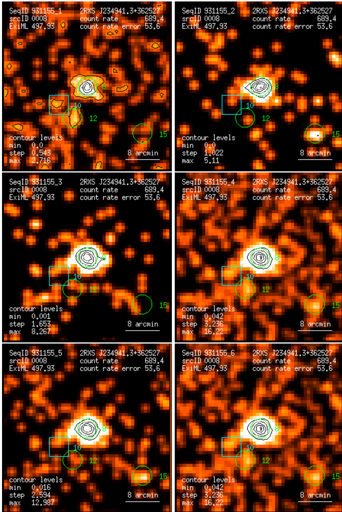
Figure 8: RASS 931155: detection 0008: band rate images, Gaussian filter: (1) PSPC channels 11 – 41, (2) 52 – 90, (3) 91 – 201, (4) 11 – 235, (5) 52 – 201, (6) 11 – 201. Broad band rates in counts/ks. Band rate contour levels in counts/ks/arcmin 2 .
