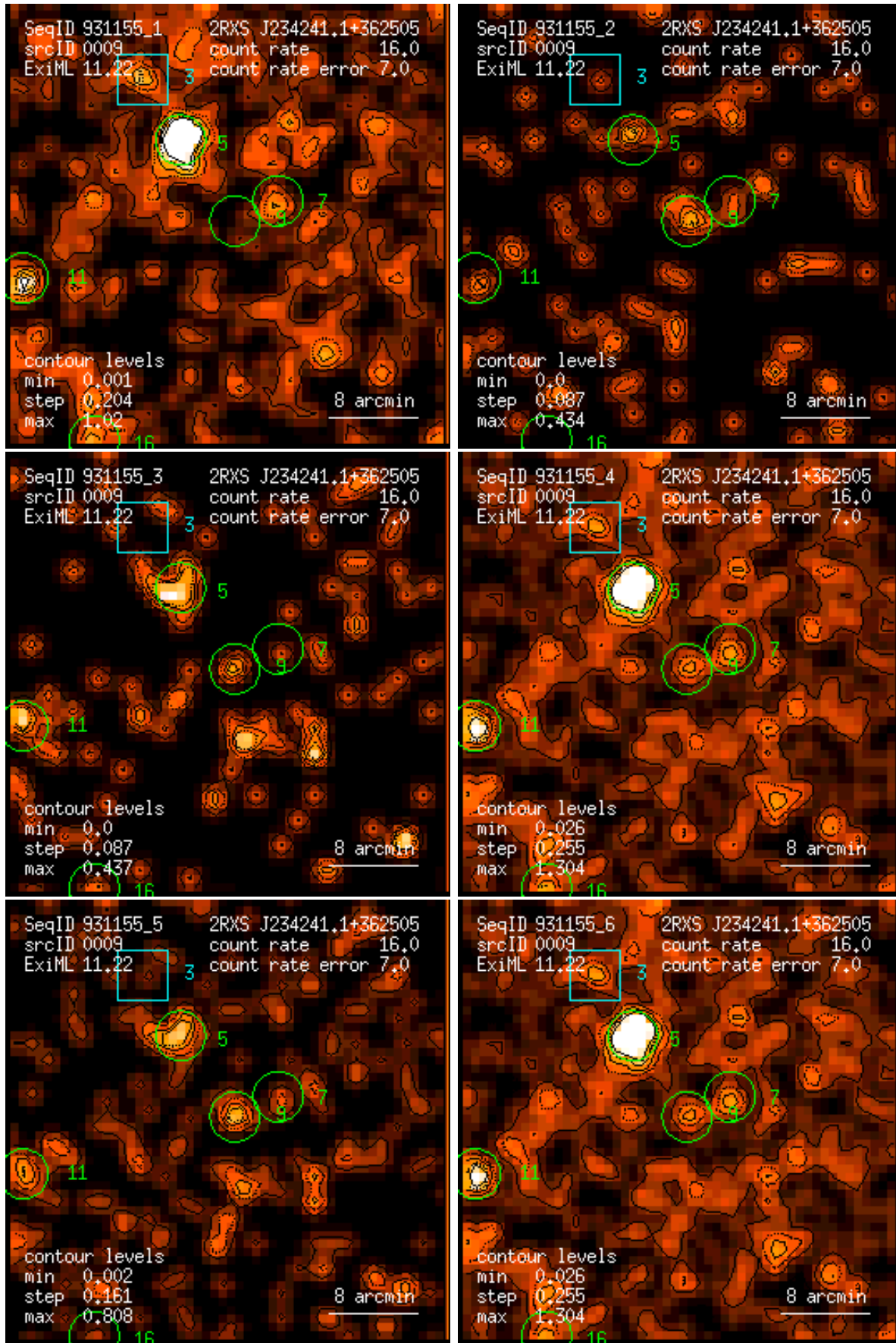
Figure 9: RASS 931155: detection 0009: band rate images, Gaussian filter: (1) PSPC channels 11 – 41, (2) 52 – 90, (3) 91 – 201, (4) 11 – 235, (5) 52 – 201, (6) 11 – 201. Broad band rates in counts/ks. Band rate contour levels in counts/ks/arcmin 2 .
