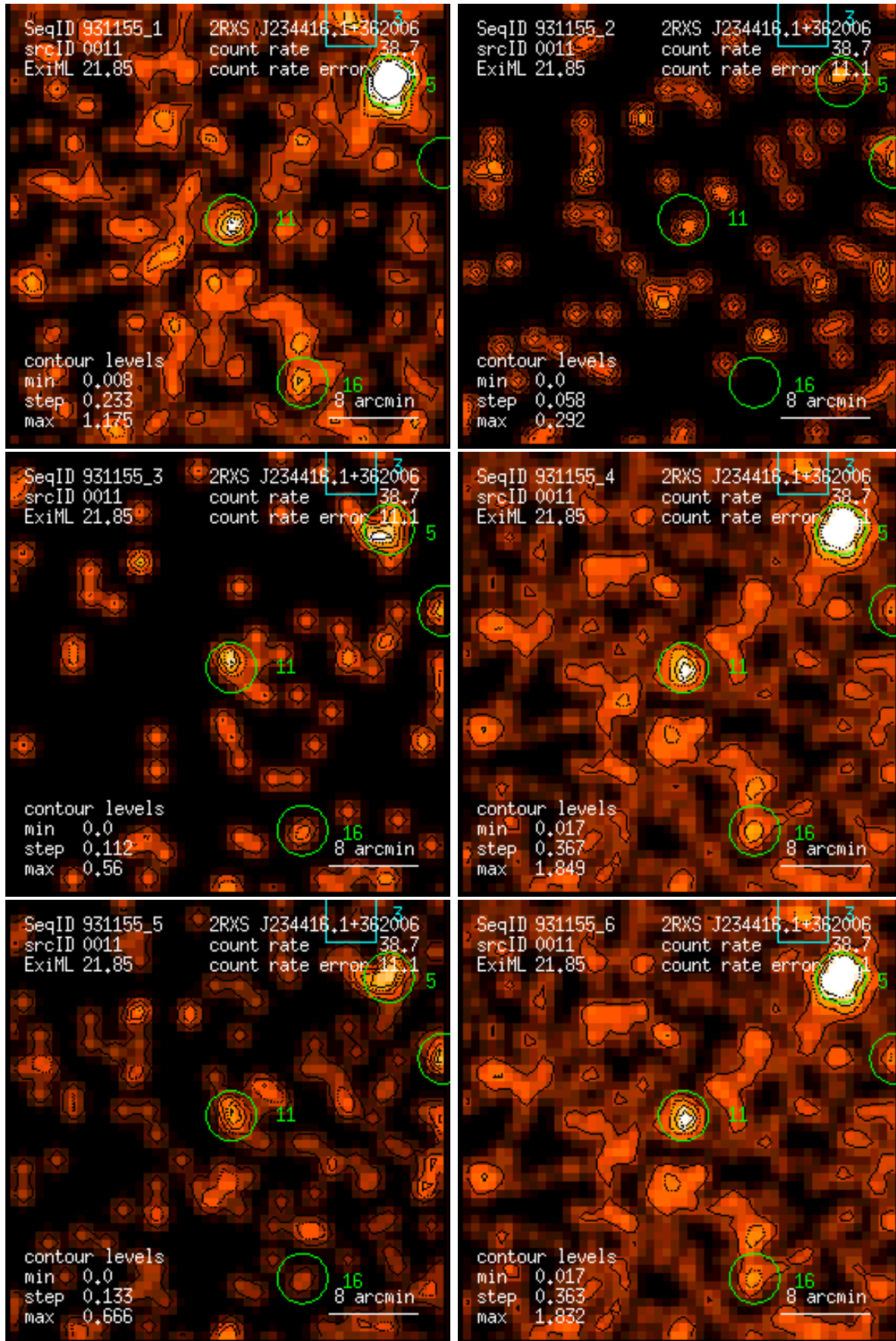
Figure 11: RASS 931155: detection 0011: band rate images, Gaussian filter: (1) PSPC channels 11 – 41, (2) 52 – 90, (3) 91 – 201, (4) 11 – 235, (5) 52 – 201, (6) 11 – 201. Broad band rates in counts/ks. Band rate contour levels in counts/ks/arcmin 2 .
