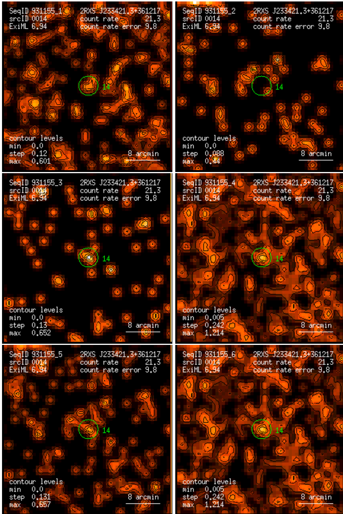
Figure 14: RASS 931155: detection 0014: band rate images, Gaussian filter: (1) PSPC channels 11 – 41, (2) 52 – 90, (3) 91 – 201, (4) 11 – 235, (5) 52 – 201, (6) 11 – 201. Broad band rates in counts/ks. Band rate contour levels in counts/ks/arcmin 2 .
