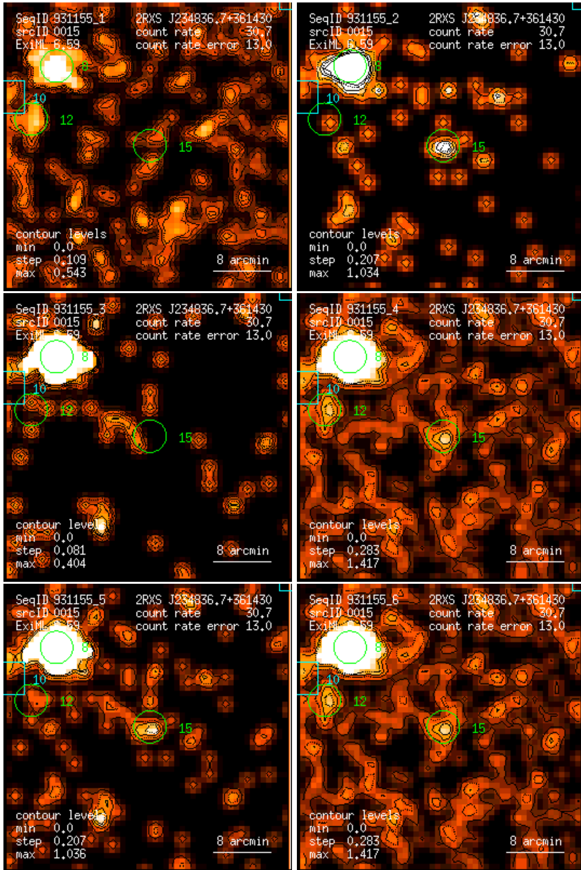
Figure 15: RASS 931155: detection 0015: band rate images, Gaussian filter: (1) PSPC channels 11 – 41, (2) 52 – 90, (3) 91 – 201, (4) 11 – 235, (5) 52 – 201, (6) 11 – 201. Broad band rates in counts/ks. Band rate contour levels in counts/ks/arcmin 2 .
