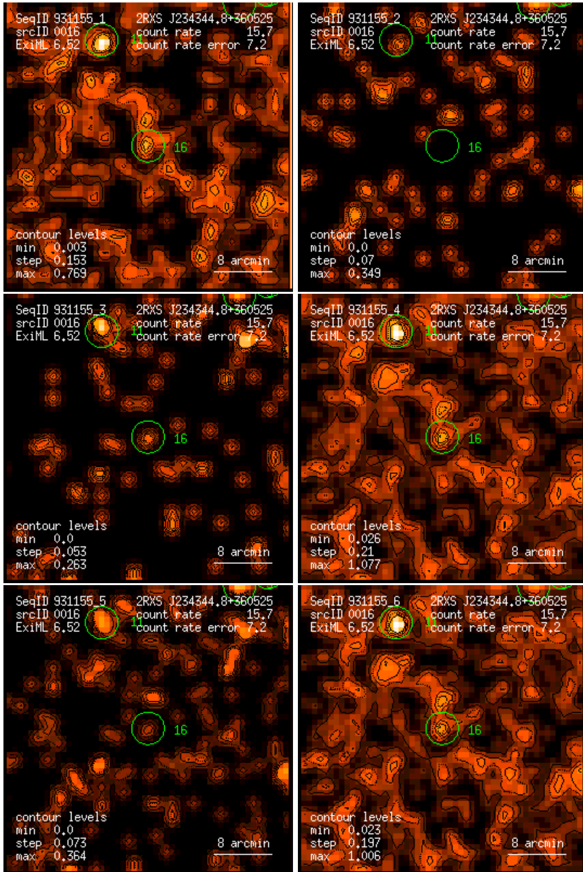
Figure 16: RASS 931155: detection 0016: band rate images, Gaussian filter: (1) PSPC channels 11 – 41, (2) 52 – 90, (3) 91 – 201, (4) 11 – 235, (5) 52 – 201, (6) 11 – 201. Broad band rates in counts/ks. Band rate contour levels in counts/ks/arcmin 2 .
