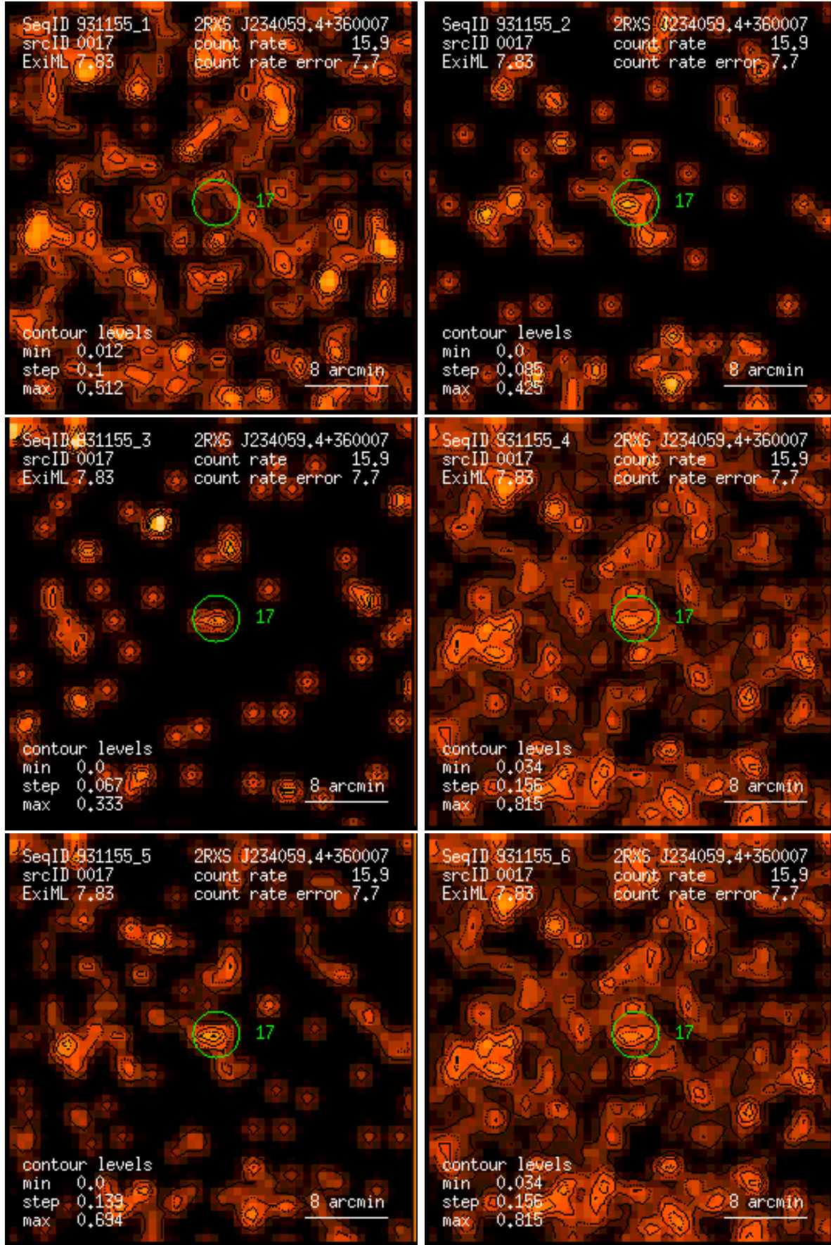
Figure 17: RASS 931155: detection 0017: band rate images, Gaussian filter: (1) PSPC channels 11 – 41, (2) 52 – 90, (3) 91 – 201, (4) 11 – 235, (5) 52 – 201, (6) 11 – 201. Broad band rates in counts/ks. Band rate contour levels in counts/ks/arcmin 2 .
