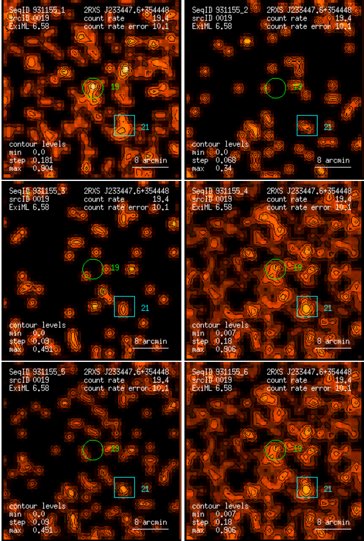
Figure 19: RASS 931155: detection 0019: band rate images, Gaussian filter: (1) PSPC channels 11 – 41, (2) 52 – 90, (3) 91 – 201, (4) 11 – 235, (5) 52 – 201, (6) 11 – 201. Broad band rates in counts/ks. Band rate contour levels in counts/ks/arcmin 2 .
