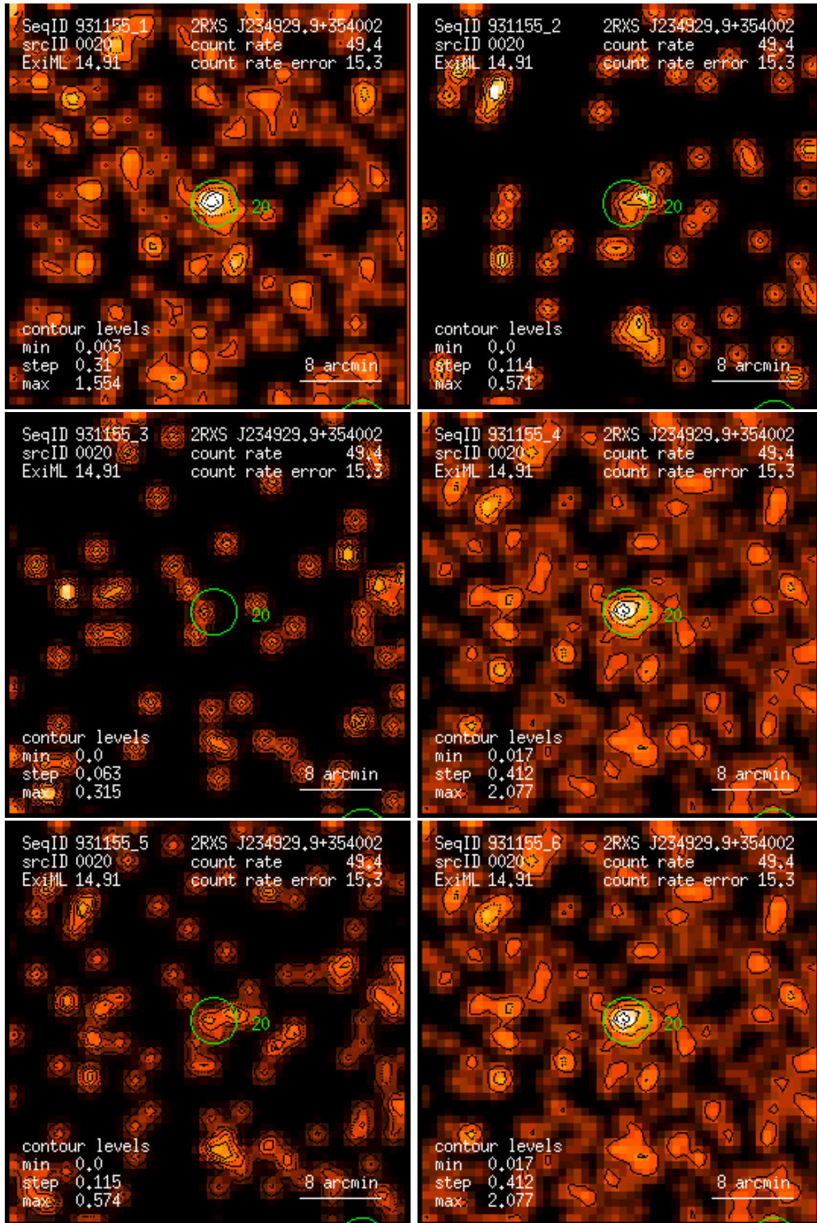
Figure 20: RASS 931155: detection 0020: band rate images, Gaussian filter: (1) PSPC channels 11 – 41, (2) 52 – 90, (3) 91 – 201, (4) 11 – 235, (5) 52 – 201, (6) 11 – 201. Broad band rates in counts/ks. Band rate contour levels in counts/ks/arcmin 2 .
