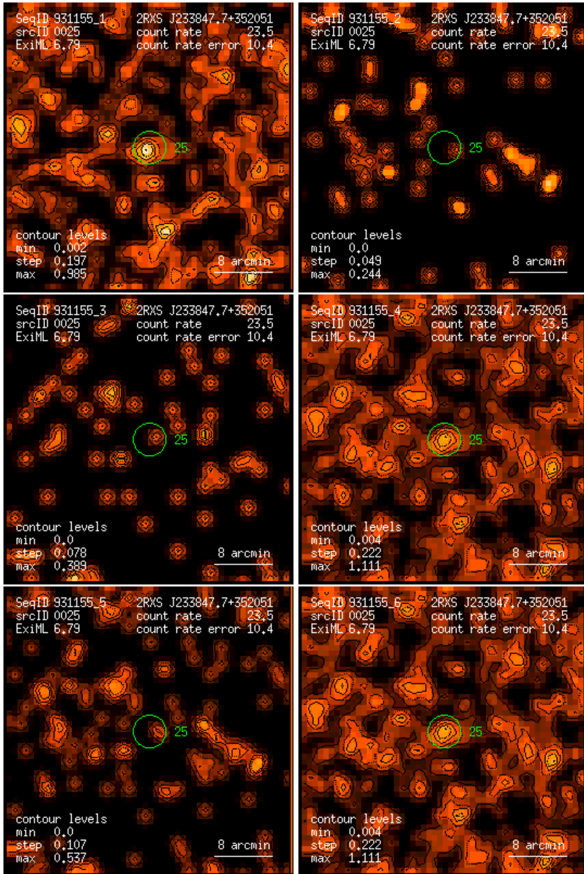
Figure 25: RASS 931155: detection 0025: band rate images, Gaussian filter: (1) PSPC channels 11 – 41, (2) 52 – 90, (3) 91 – 201, (4) 11 – 235, (5) 52 – 201, (6) 11 – 201. Broad band rates in counts/ks. Band rate contour levels in counts/ks/arcmin 2 .
