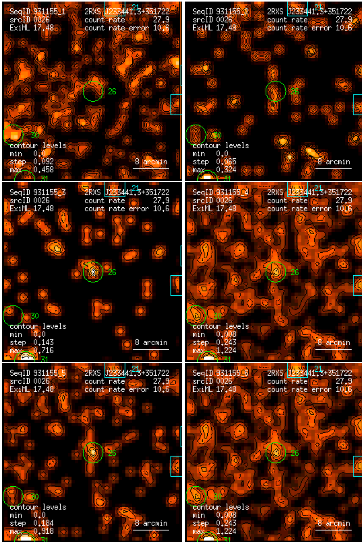
Figure 26: RASS 931155: detection 0026: band rate images, Gaussian filter: (1) PSPC channels 11 – 41, (2) 52 – 90, (3) 91 – 201, (4) 11 – 235, (5) 52 – 201, (6) 11 – 201. Broad band rates in counts/ks. Band rate contour levels in counts/ks/arcmin 2 .
