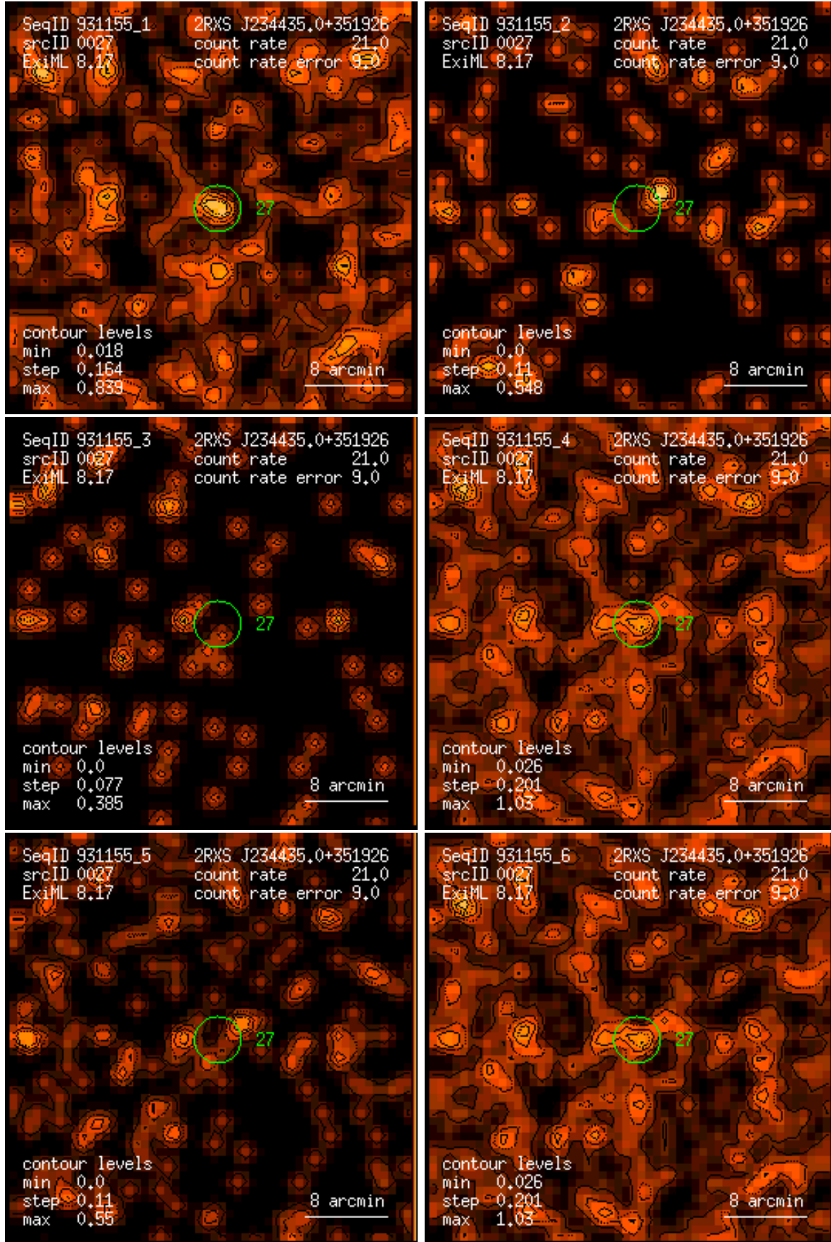
Figure 27: RASS 931155: detection 0027: band rate images, Gaussian filter: (1) PSPC channels 11 – 41, (2) 52 – 90, (3) 91 – 201, (4) 11 – 235, (5) 52 – 201, (6) 11 – 201. Broad band rates in counts/ks. Band rate contour levels in counts/ks/arcmin 2 .
