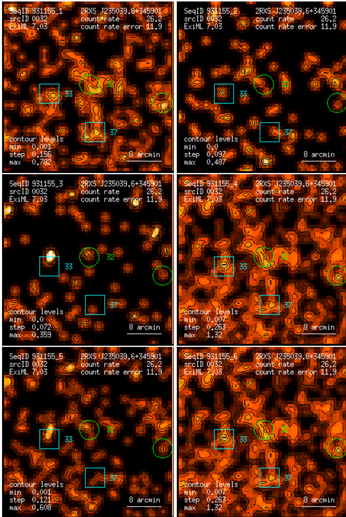
Figure 32: RASS 931155: detection 0032: band rate images, Gaussian filter: (1) PSPC channels 11 – 41, (2) 52 – 90, (3) 91 – 201, (4) 11 – 235, (5) 52 – 201, (6) 11 – 201. Broad band rates in counts/ks. Band rate contour levels in counts/ks/arcmin 2 .
