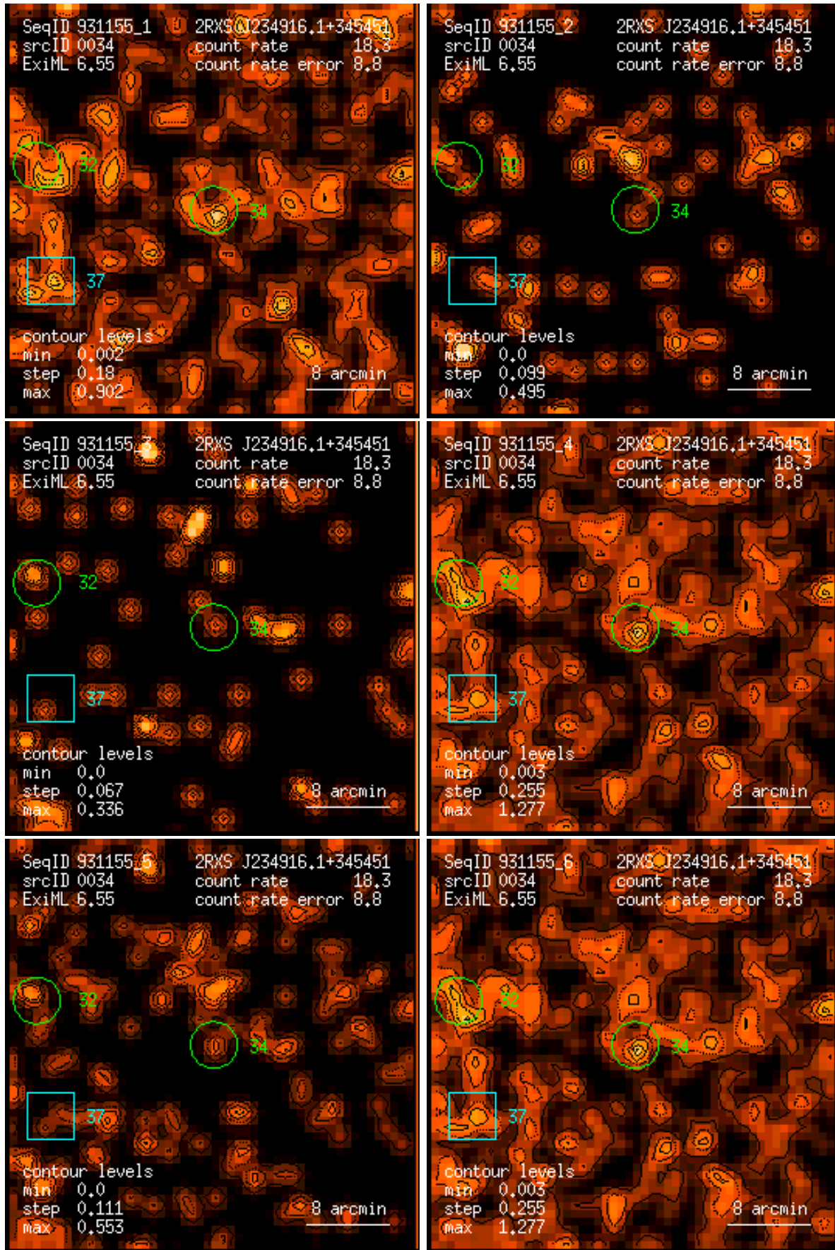
Figure 34: RASS 931155: detection 0034: band rate images, Gaussian filter: (1) PSPC channels 11 – 41, (2) 52 – 90, (3) 91 – 201, (4) 11 – 235, (5) 52 – 201, (6) 11 – 201. Broad band rates in counts/ks. Band rate contour levels in counts/ks/arcmin 2 .
