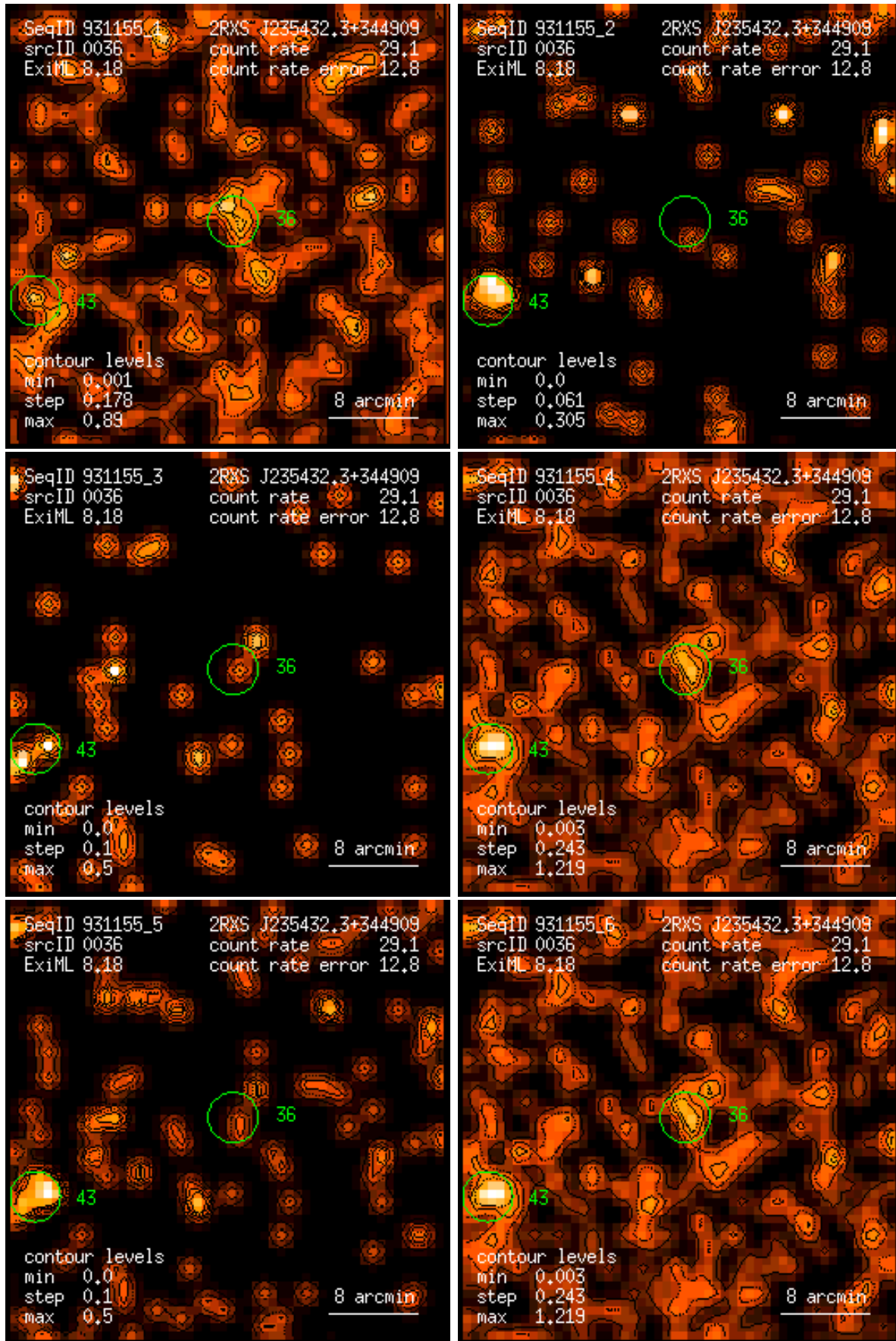
Figure 36: RASS 931155: detection 0036: band rate images, Gaussian filter: (1) PSPC channels 11 – 41, (2) 52 – 90, (3) 91 – 201, (4) 11 – 235, (5) 52 – 201, (6) 11 – 201. Broad band rates in counts/ks. Band rate contour levels in counts/ks/arcmin 2 .
