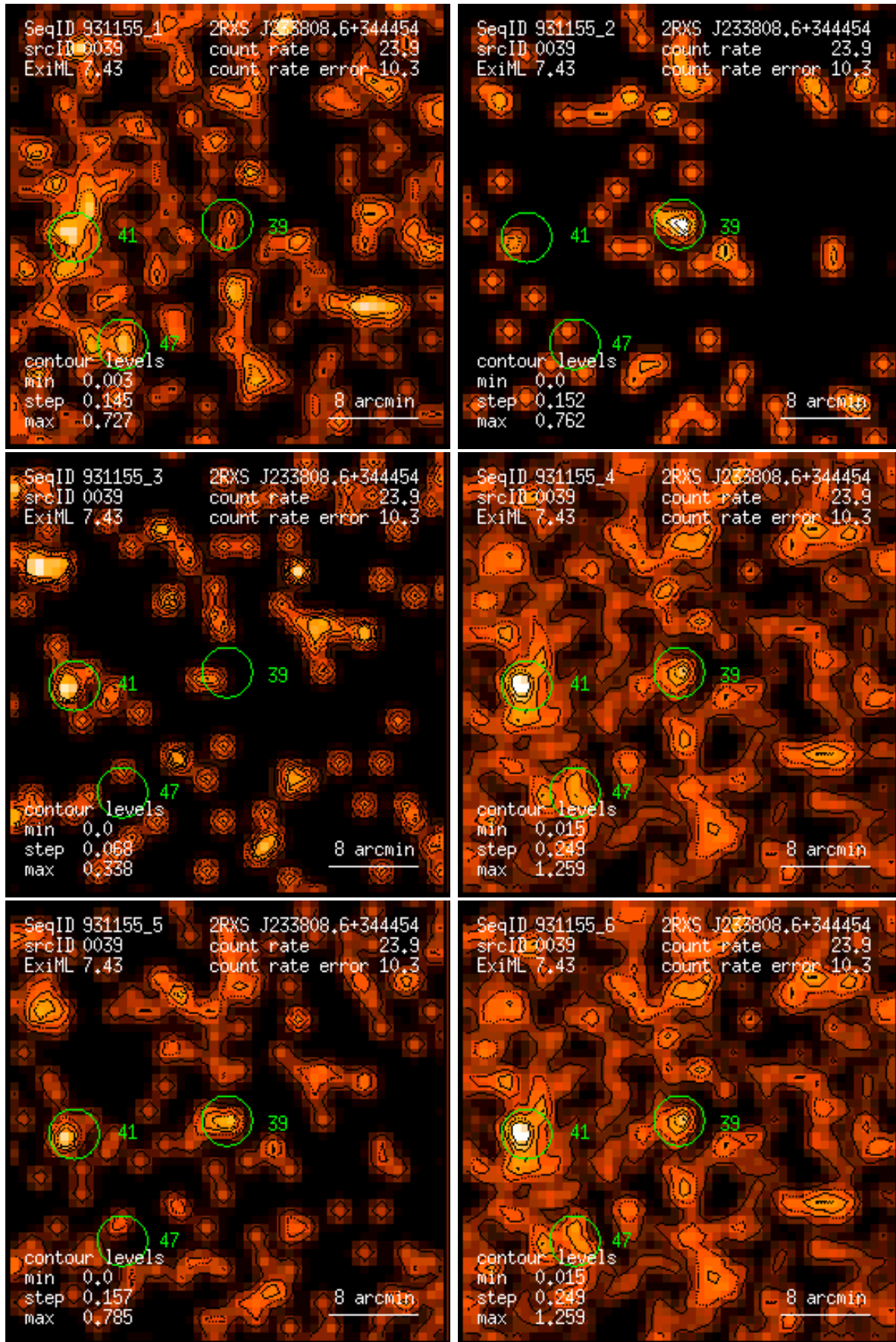
Figure 39: RASS 931155: detection 0039: band rate images, Gaussian filter: (1) PSPC channels 11 – 41, (2) 52 – 90, (3) 91 – 201, (4) 11 – 235, (5) 52 – 201, (6) 11 – 201. Broad band rates in counts/ks. Band rate contour levels in counts/ks/arcmin 2 .
