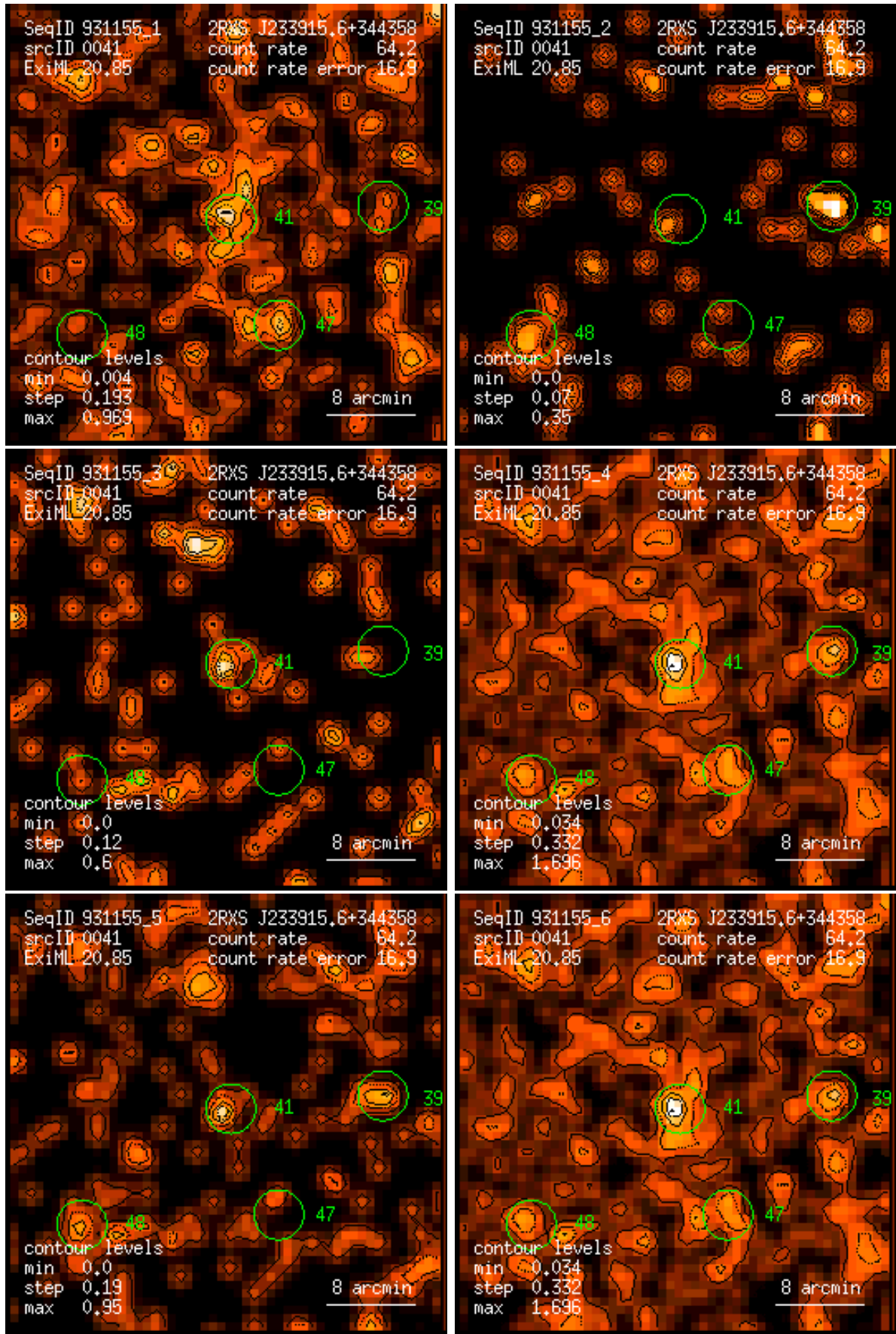
Figure 41: RASS 931155: detection 0041: band rate images, Gaussian filter: (1) PSPC channels 11 – 41, (2) 52 – 90, (3) 91 – 201, (4) 11 – 235, (5) 52 – 201, (6) 11 – 201. Broad band rates in counts/ks. Band rate contour levels in counts/ks/arcmin 2 .
