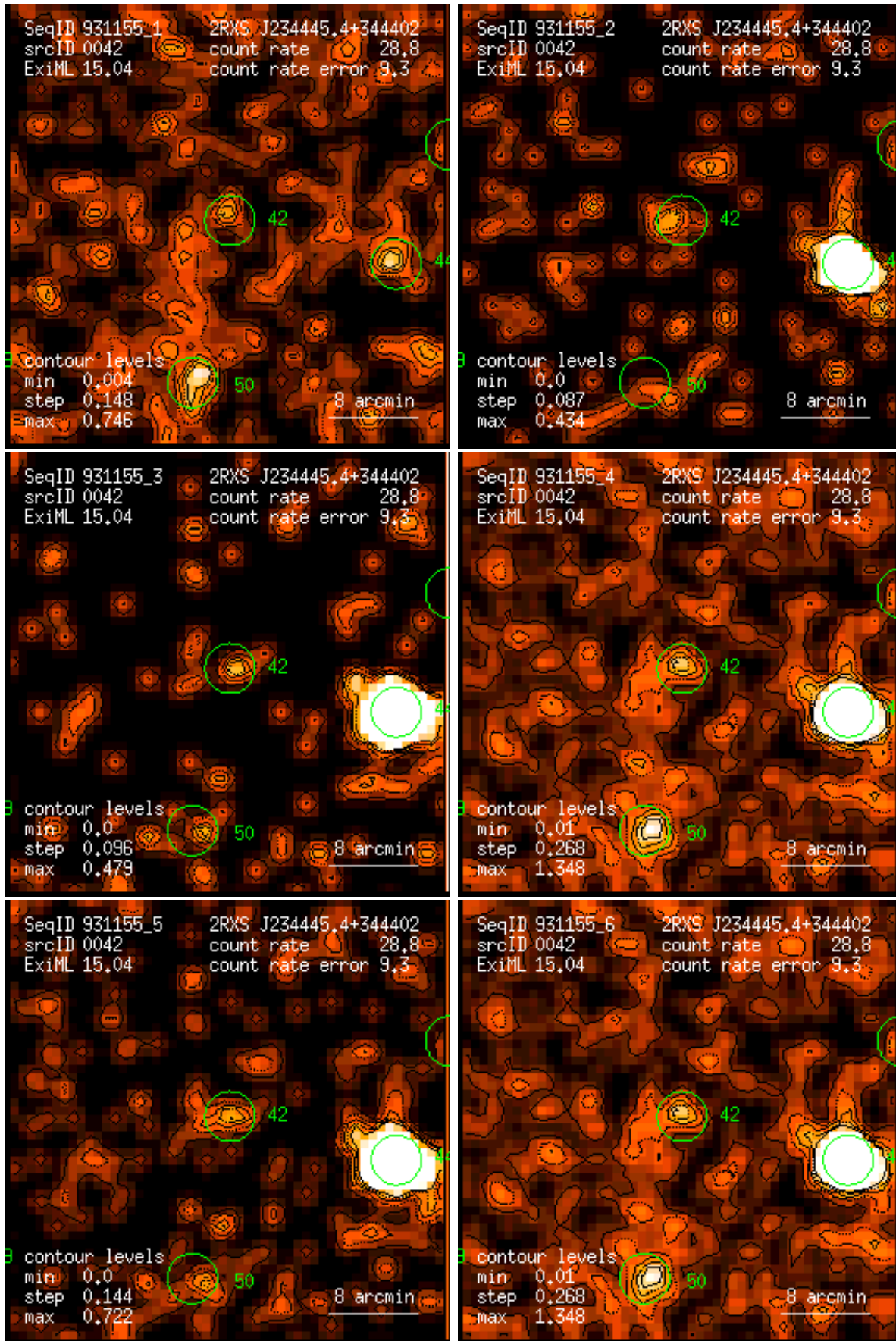
Figure 42: RASS 931155: detection 0042: band rate images, Gaussian filter: (1) PSPC channels 11 – 41, (2) 52 – 90, (3) 91 – 201, (4) 11 – 235, (5) 52 – 201, (6) 11 – 201. Broad band rates in counts/ks. Band rate contour levels in counts/ks/arcmin 2 .
