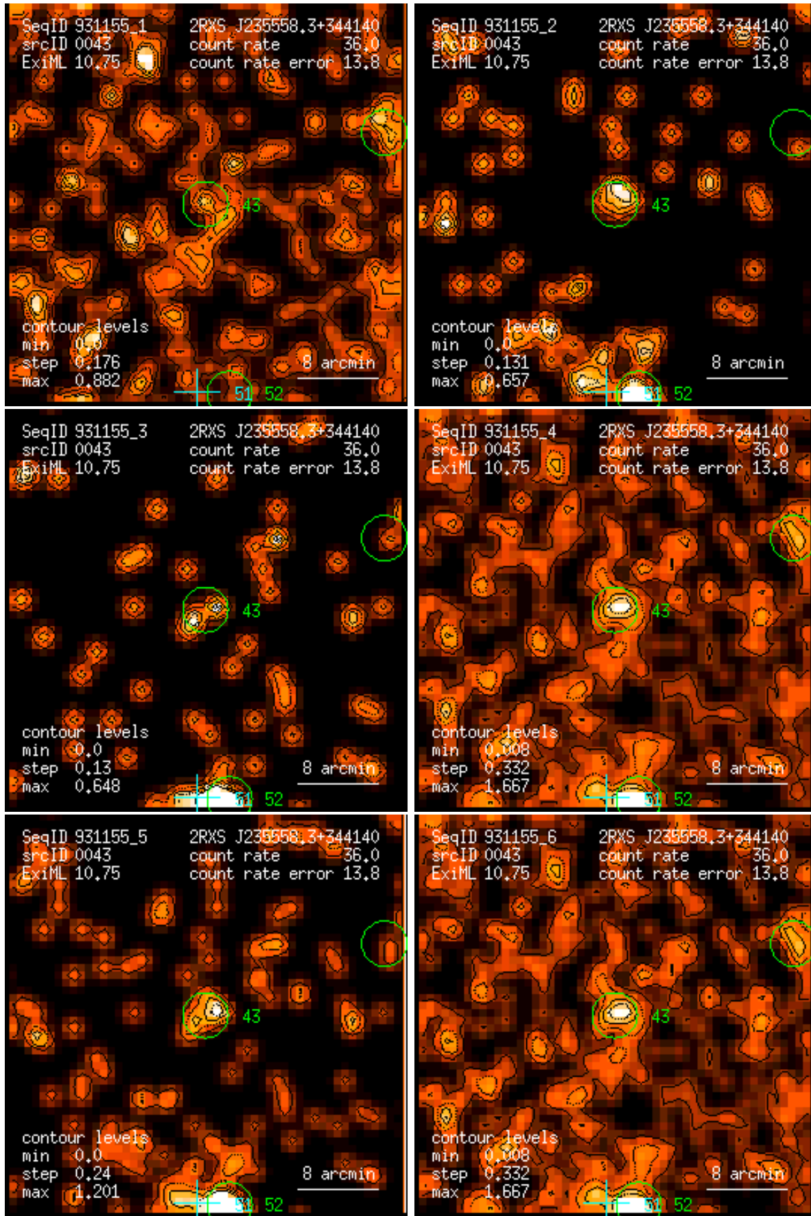
Figure 43: RASS 931155: detection 0043: band rate images, Gaussian filter: (1) PSPC channels 11 – 41, (2) 52 – 90, (3) 91 – 201, (4) 11 – 235, (5) 52 – 201, (6) 11 – 201. Broad band rates in counts/ks. Band rate contour levels in counts/ks/arcmin 2 .
