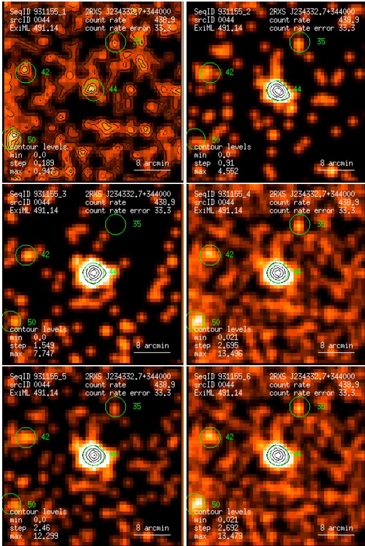
Figure 44: RASS 931155: detection 0044: band rate images, Gaussian filter: (1) PSPC channels 11 – 41, (2) 52 – 90, (3) 91 – 201, (4) 11 – 235, (5) 52 – 201, (6) 11 – 201. Broad band rates in counts/ks. Band rate contour levels in counts/ks/arcmin 2 .
