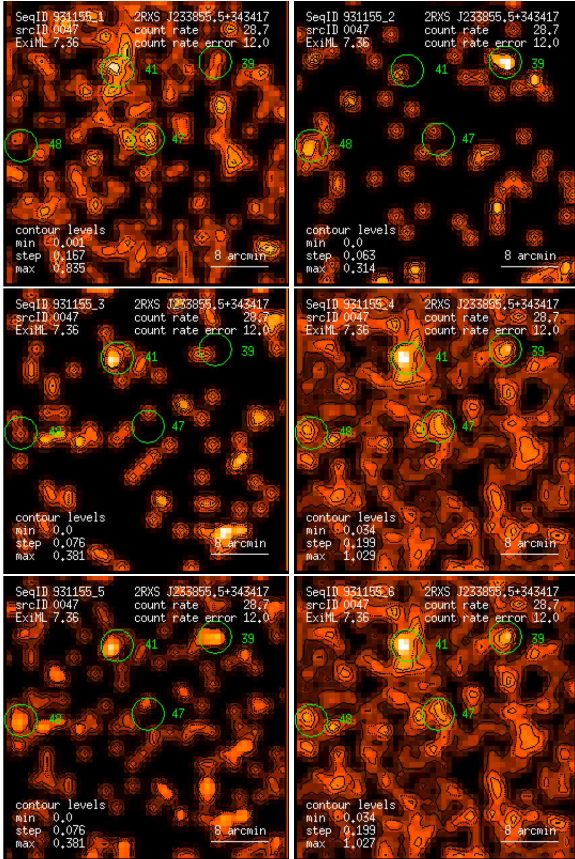
Figure 47: RASS 931155: detection 0047: band rate images, Gaussian filter: (1) PSPC channels 11 – 41, (2) 52 – 90, (3) 91 – 201, (4) 11 – 235, (5) 52 – 201, (6) 11 – 201. Broad band rates in counts/ks. Band rate contour levels in counts/ks/arcmin 2 .
