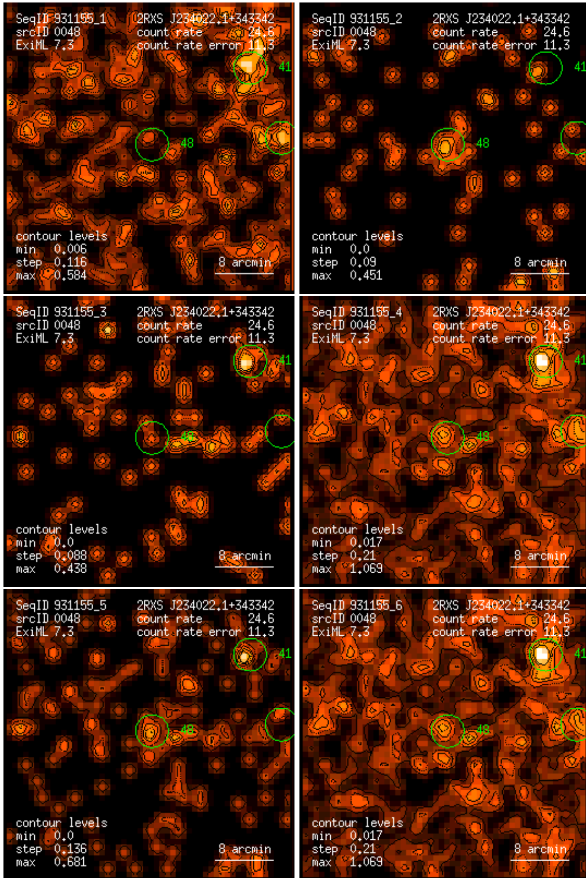
Figure 48: RASS 931155: detection 0048: band rate images, Gaussian filter: (1) PSPC channels 11 – 41, (2) 52 – 90, (3) 91 – 201, (4) 11 – 235, (5) 52 – 201, (6) 11 – 201. Broad band rates in counts/ks. Band rate contour levels in counts/ks/arcmin 2 .
