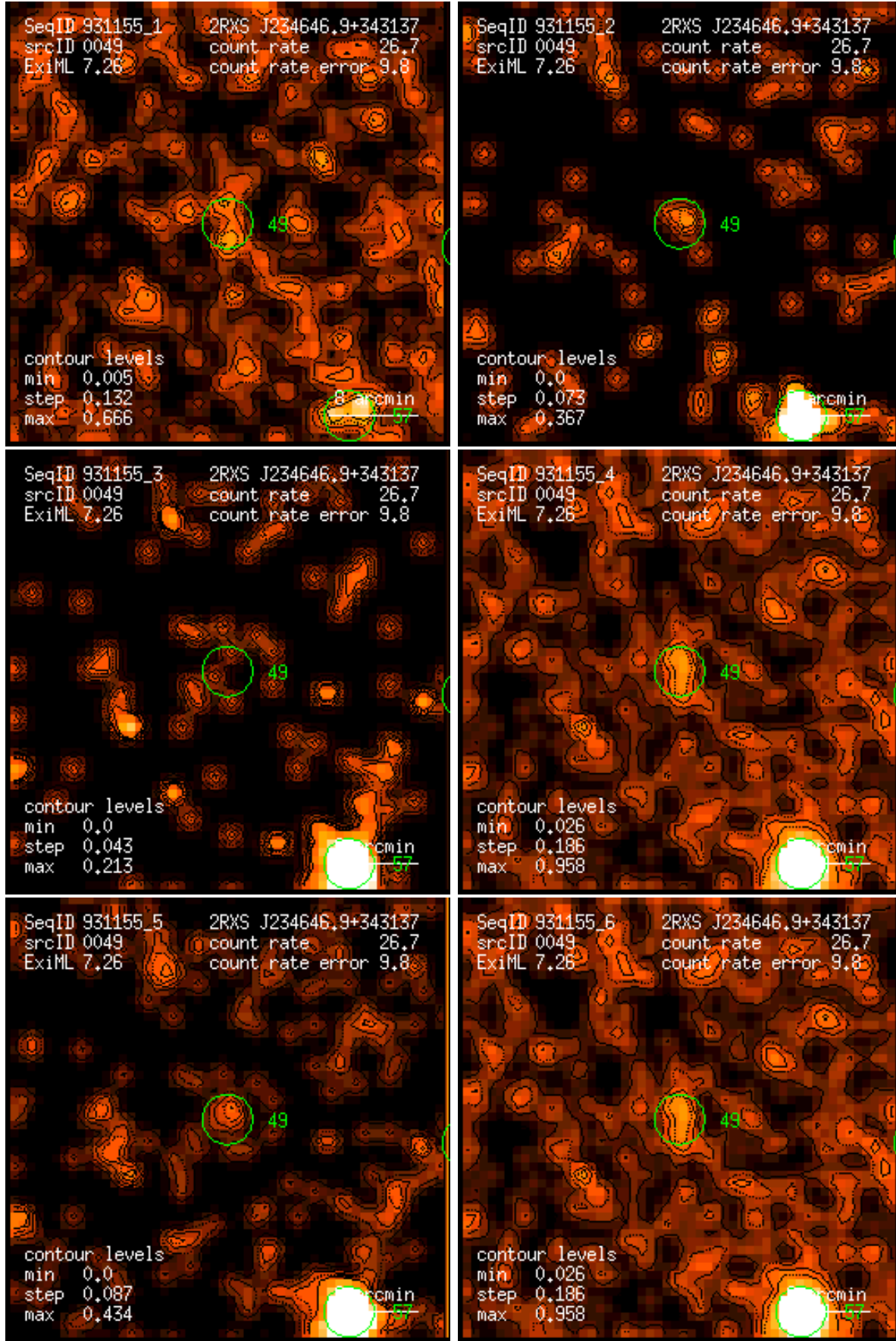
Figure 49: RASS 931155: detection 0049: band rate images, Gaussian filter: (1) PSPC channels 11 – 41, (2) 52 – 90, (3) 91 – 201, (4) 11 – 235, (5) 52 – 201, (6) 11 – 201. Broad band rates in counts/ks. Band rate contour levels in counts/ks/arcmin 2 .
