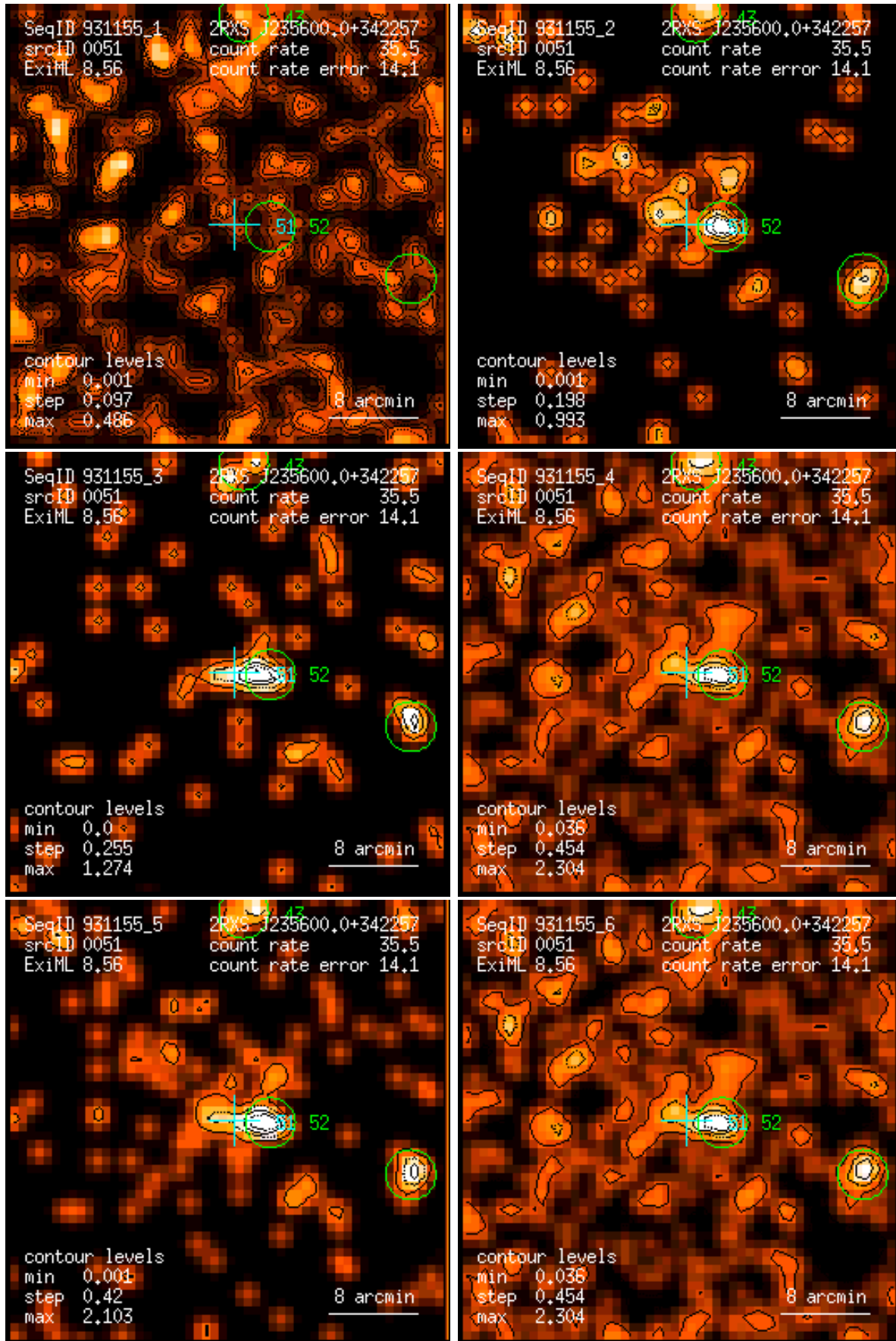
Figure 51: RASS 931155: detection 0051: band rate images, Gaussian filter: (1) PSPC channels 11 – 41, (2) 52 – 90, (3) 91 – 201, (4) 11 – 235, (5) 52 – 201, (6) 11 – 201. Broad band rates in counts/ks. Band rate contour levels in counts/ks/arcmin 2 .
