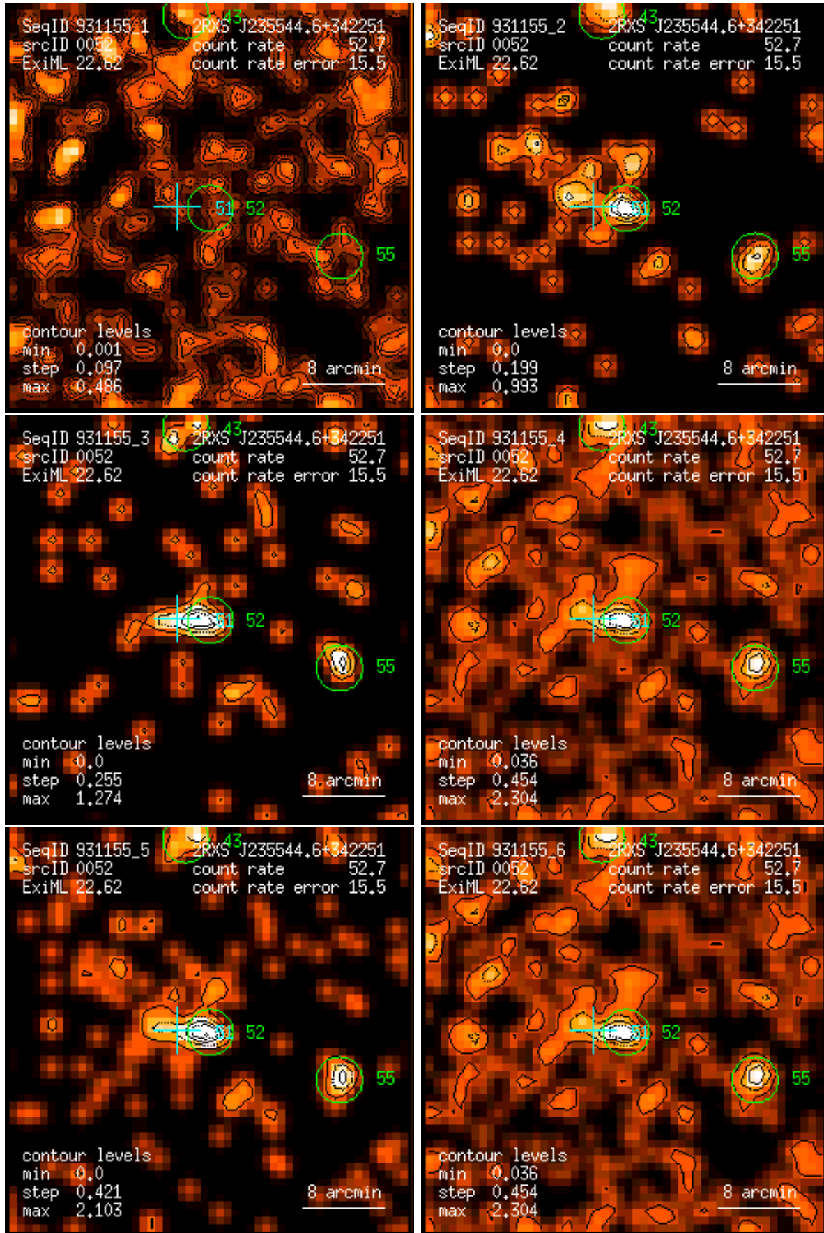
Figure 52: RASS 931155: detection 0052: band rate images, Gaussian filter: (1) PSPC channels 11 – 41, (2) 52 – 90, (3) 91 – 201, (4) 11 – 235, (5) 52 – 201, (6) 11 – 201. Broad band rates in counts/ks. Band rate contour levels in counts/ks/arcmin 2 .
