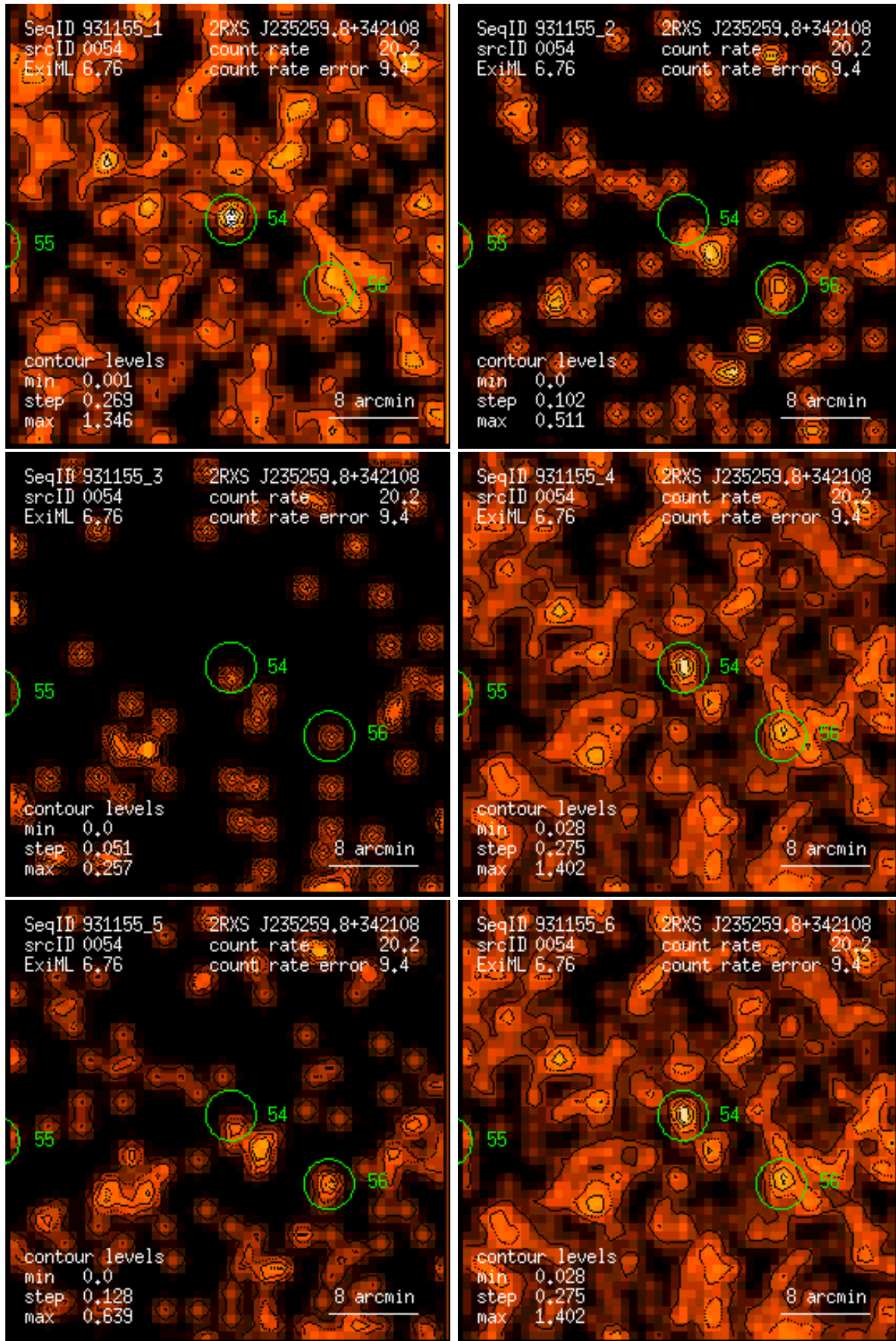
Figure 54: RASS 931155: detection 0054: band rate images, Gaussian filter: (1) PSPC channels 11 – 41, (2) 52 – 90, (3) 91 – 201, (4) 11 – 235, (5) 52 – 201, (6) 11 – 201. Broad band rates in counts/ks. Band rate contour levels in counts/ks/arcmin 2 .
