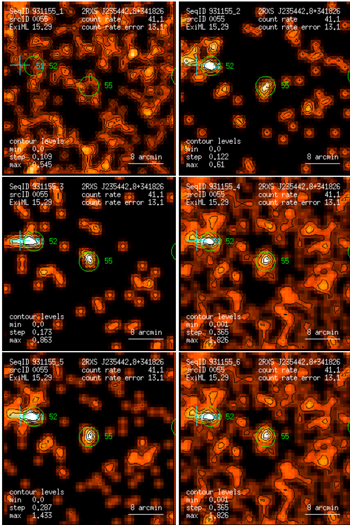
Figure 55: RASS 931155: detection 0055: band rate images, Gaussian filter: (1) PSPC channels 11 – 41, (2) 52 – 90, (3) 91 – 201, (4) 11 – 235, (5) 52 – 201, (6) 11 – 201. Broad band rates in counts/ks. Band rate contour levels in counts/ks/arcmin 2 .
