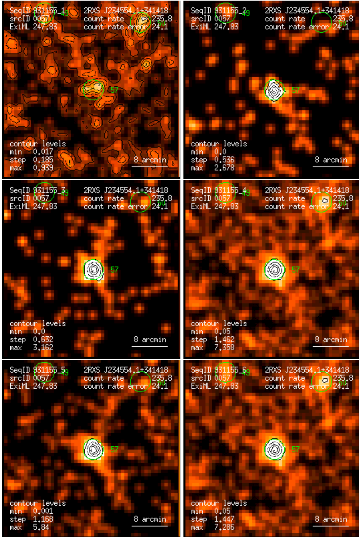
Figure 57: RASS 931155: detection 0057: band rate images, Gaussian filter: (1) PSPC channels 11 – 41, (2) 52 – 90, (3) 91 – 201, (4) 11 – 235, (5) 52 – 201, (6) 11 – 201. Broad band rates in counts/ks. Band rate contour levels in counts/ks/arcmin 2 .
