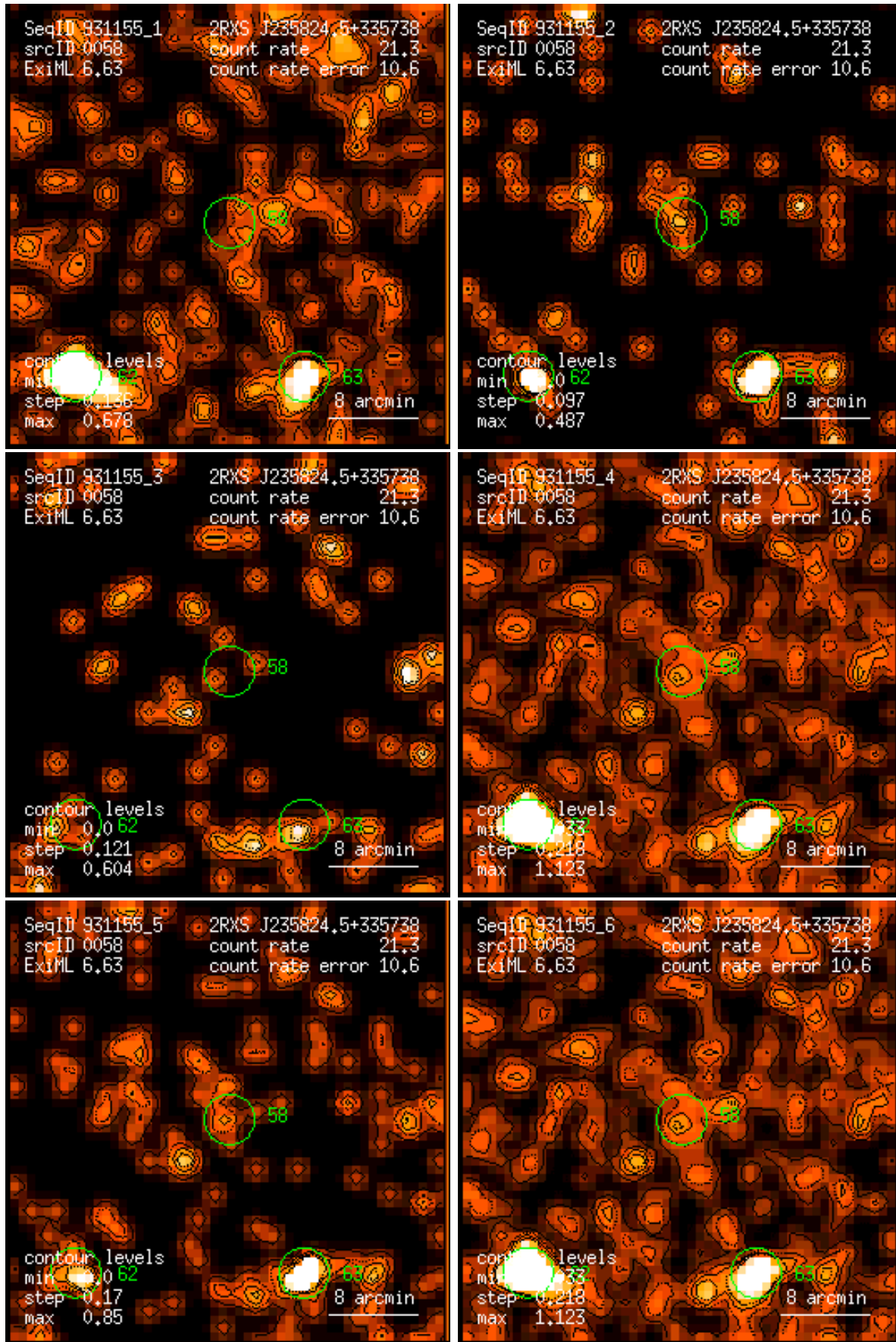
Figure 58: RASS 931155: detection 0058: band rate images, Gaussian filter: (1) PSPC channels 11 – 41, (2) 52 – 90, (3) 91 – 201, (4) 11 – 235, (5) 52 – 201, (6) 11 – 201. Broad band rates in counts/ks. Band rate contour levels in counts/ks/arcmin 2 .
