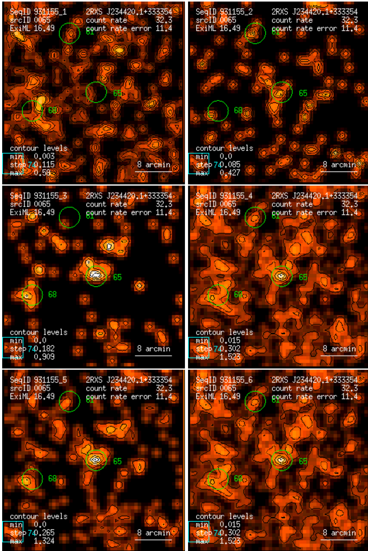
Figure 65: RASS 931155: detection 0065: band rate images, Gaussian filter: (1) PSPC channels 11 – 41, (2) 52 – 90, (3) 91 – 201, (4) 11 – 235, (5) 52 – 201, (6) 11 – 201. Broad band rates in counts/ks. Band rate contour levels in counts/ks/arcmin 2 .
