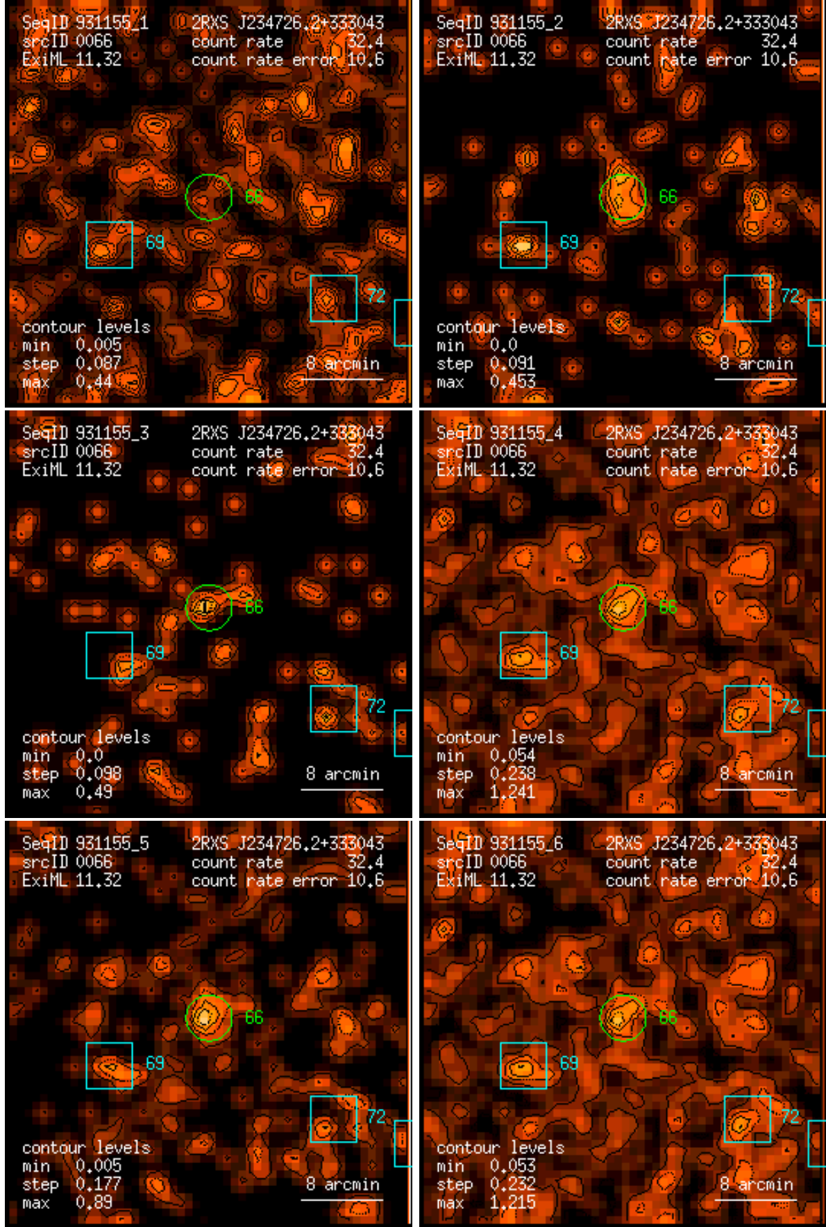
Figure 66: RASS 931155: detection 0066: band rate images, Gaussian filter: (1) PSPC channels 11 – 41, (2) 52 – 90, (3) 91 – 201, (4) 11 – 235, (5) 52 – 201, (6) 11 – 201. Broad band rates in counts/ks. Band rate contour levels in counts/ks/arcmin 2 .
