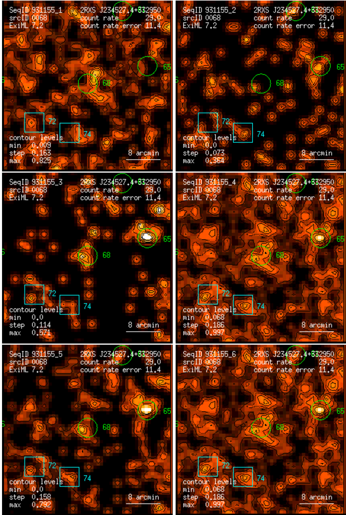
Figure 68: RASS 931155: detection 0068: band rate images, Gaussian filter: (1) PSPC channels 11 – 41, (2) 52 – 90, (3) 91 – 201, (4) 11 – 235, (5) 52 – 201, (6) 11 – 201. Broad band rates in counts/ks. Band rate contour levels in counts/ks/arcmin 2 .
