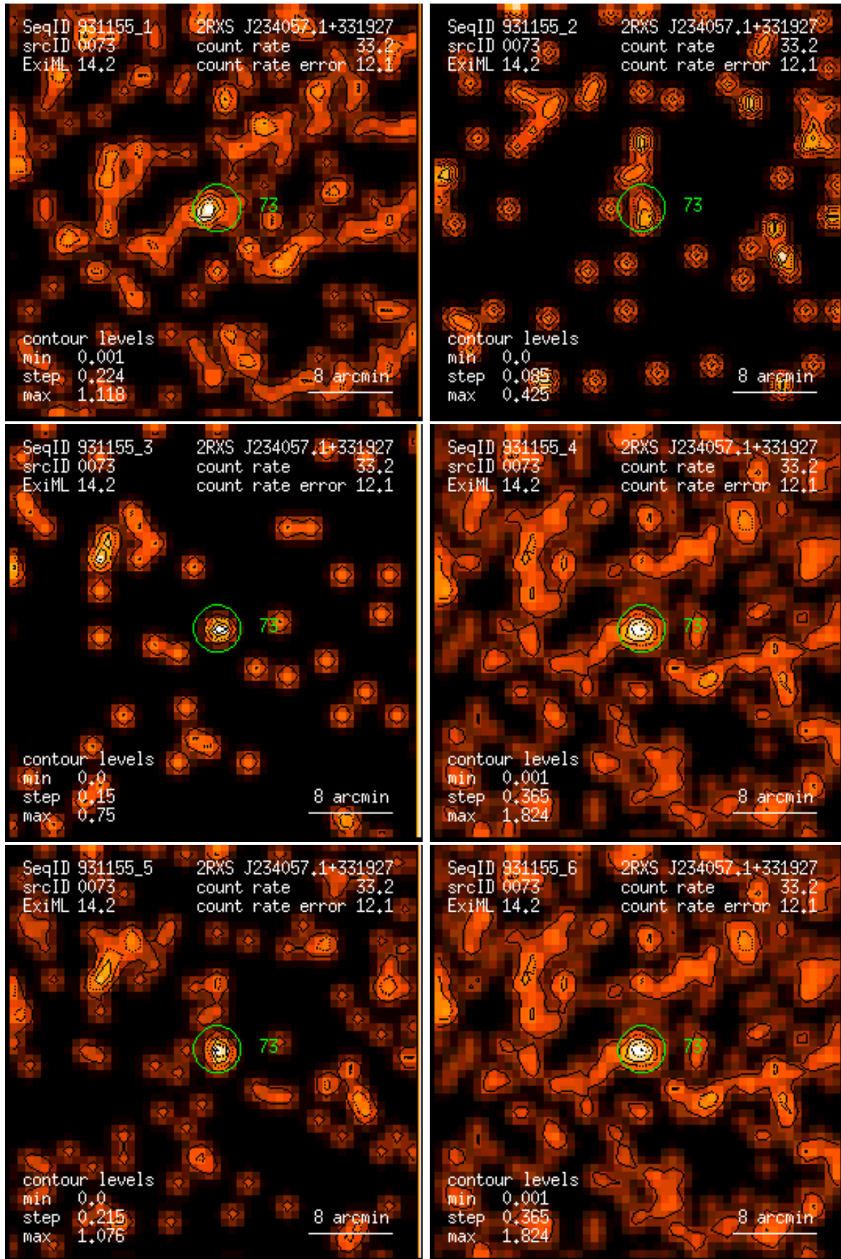
Figure 73: RASS 931155: detection 0073: band rate images, Gaussian filter: (1) PSPC channels 11 – 41, (2) 52 – 90, (3) 91 – 201, (4) 11 – 235, (5) 52 – 201, (6) 11 – 201. Broad band rates in counts/ks. Band rate contour levels in counts/ks/arcmin 2 .
