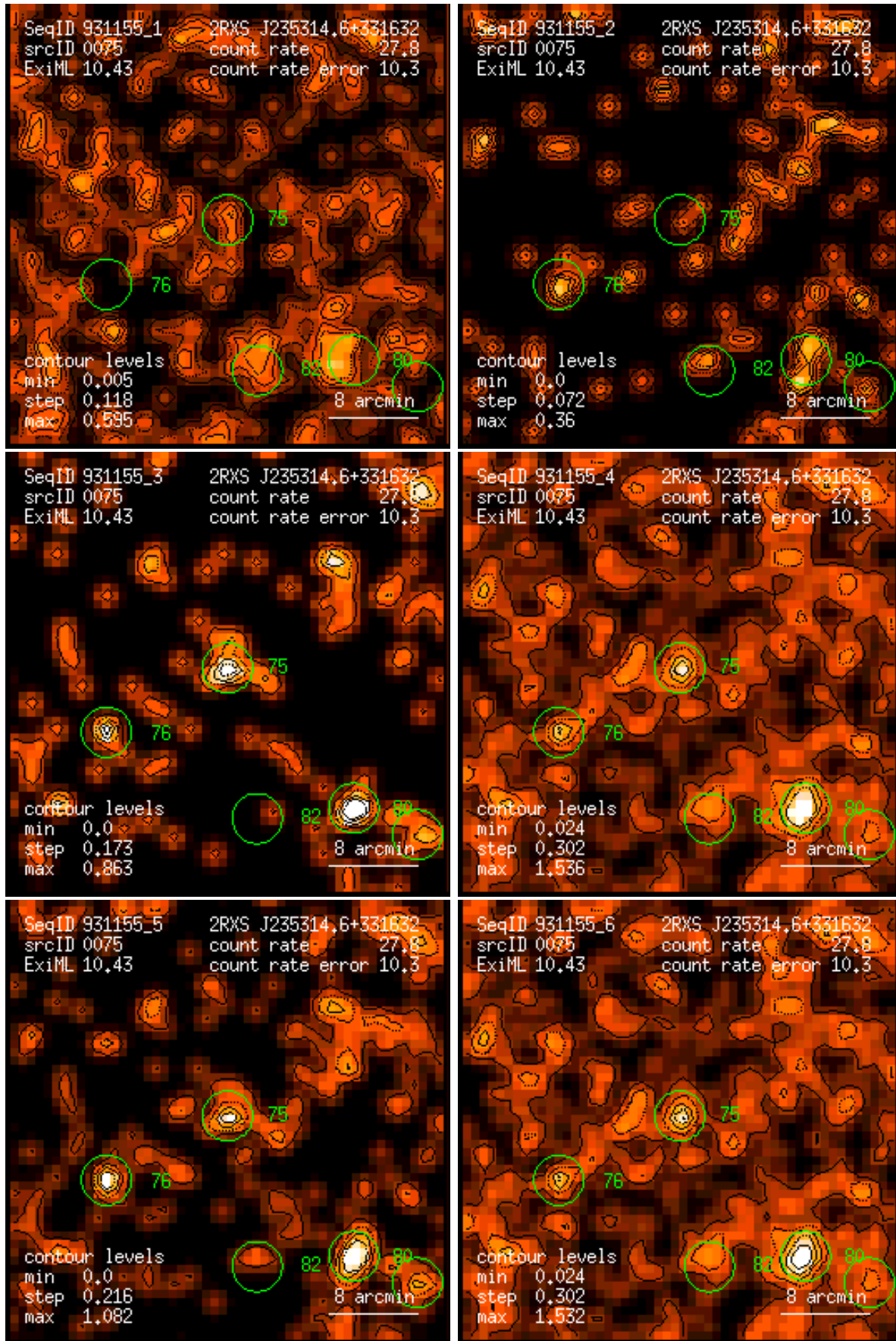
Figure 75: RASS 931155: detection 0075: band rate images, Gaussian filter: (1) PSPC channels 11 – 41, (2) 52 – 90, (3) 91 – 201, (4) 11 – 235, (5) 52 – 201, (6) 11 – 201. Broad band rates in counts/ks. Band rate contour levels in counts/ks/arcmin 2 .
