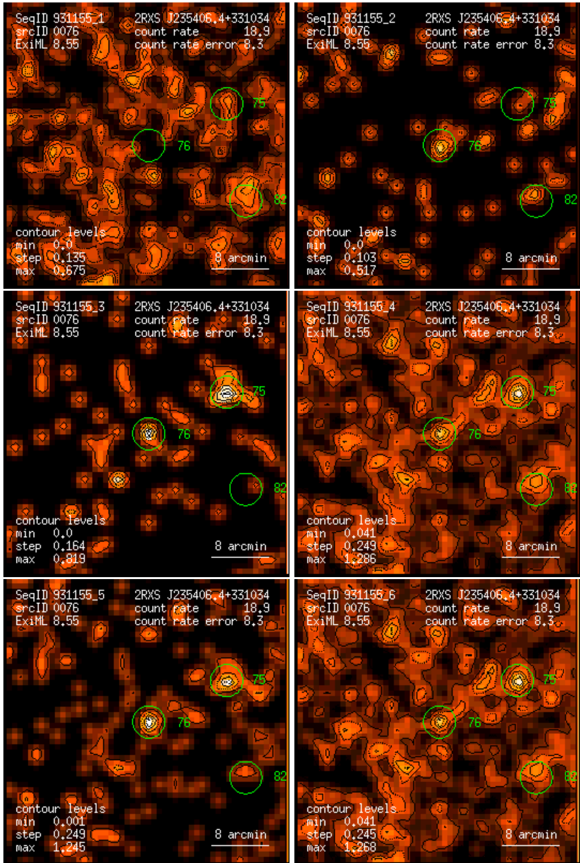
Figure 76: RASS 931155: detection 0076: band rate images, Gaussian filter: (1) PSPC channels 11 – 41, (2) 52 – 90, (3) 91 – 201, (4) 11 – 235, (5) 52 – 201, (6) 11 – 201. Broad band rates in counts/ks. Band rate contour levels in counts/ks/arcmin 2 .
